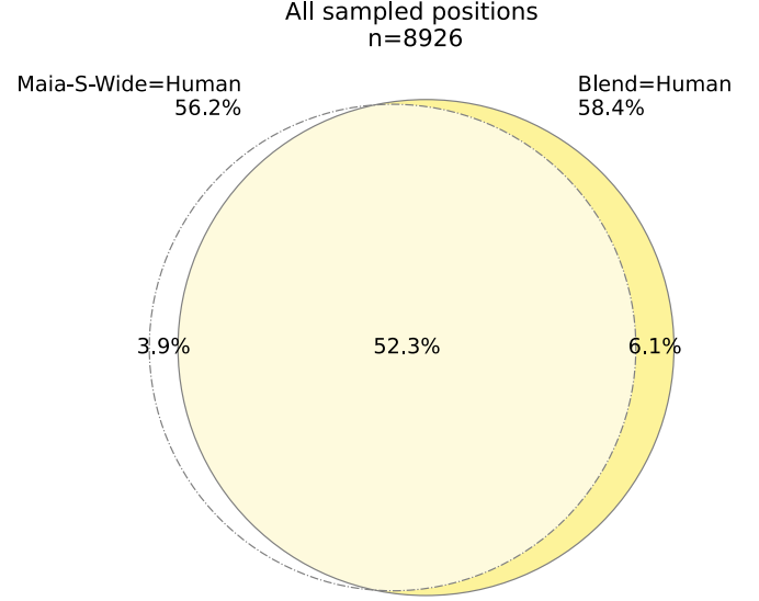
Fig. 9. Venn diagram of Maia-S-Wide and the Blend model's prediction results of the all experimented positions.
