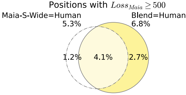
Fig. 10. Venn diagram of Maia-S-Wide and the Blend model’s prediction results of the experimented positions with Loss_{Maia} \geq 500 .
