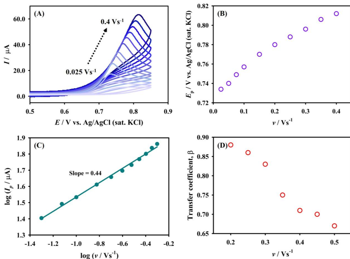
Figure 7. (A) CVs of As(III) oxidation recorded using (Pt-Au) 8 electrode for 2 mM As(III) prepared in 0.1 M H 2 SO 4 solution at variable scan rates (from 0.025 to 0.4 V s -1 ). (B) Variation of peak potential ( E_p ) with change in scan rate ( \nu ). (C) Variation of logarithm of I_p with logarithm of \nu . (D) Variation of anodic transfer coefficient ( \beta ) with changing scan rate.
