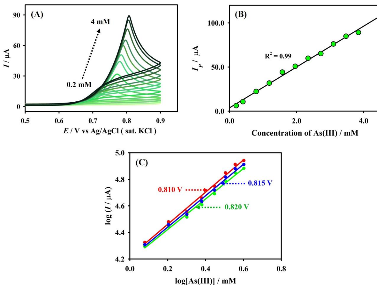
Figure 6. (A) Variation of CVs with As(III) concentration recorded using (Pt-Au) 8 electrode in 0.1 M H 2 SO 4 at a scan rate of 0.1 Vs -1 . (B) Calibration curve showing the dependence of peak
