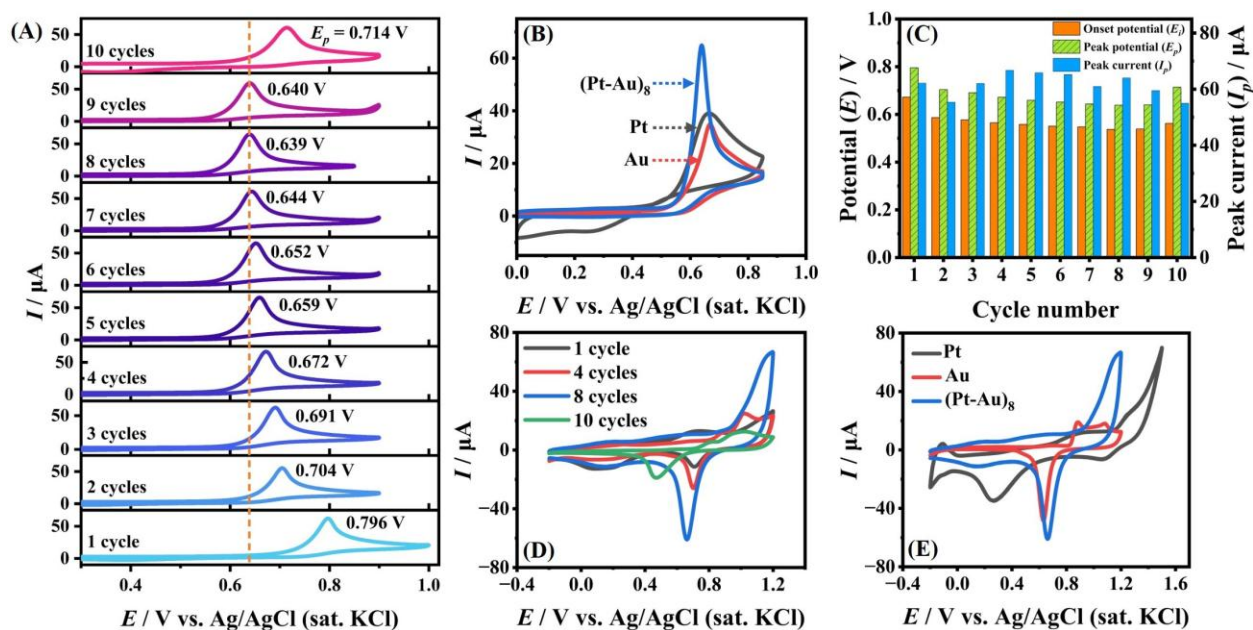
Figure 1. (A) Comparison of cyclic voltammograms (CVs) showing the performance of 1 to 10 CV cycles of Au deposition on polycrystalline Pt surface in attaining As(III) oxidation reaction. (B) Comparison of CVs among a bare Pt, a bare Au, and the (Pt-Au) 8 electrodes for As(III) oxidation reaction. (C) Bar chart demonstrating the trend in variation among onset potential ( E_i ), peak potential ( E_p ), and peak current ( I_p ) for various cycles numbers. The values in bar chart are derived from respective CVs in Figure 1A. (D) CVs recorded using Pt-Au electrode after varying Au deposition cycles on Pt in absence of arsenite solution. (E) Comparison among various characteristic CVs for a bare Pt, bare Au, and Au-modified Pt electrode in absence of arsenite solution. All the CVs were obtained at a scan rate of 0.1 Vs -1 . Arsenite oxidation performance of different electrodes were obtained by pipetting 200 \mu L of 0.1 M As(III) into a 10 mL 0.1 M H 2 SO 4 , achieving a final concentration of 2 mM As(III).
