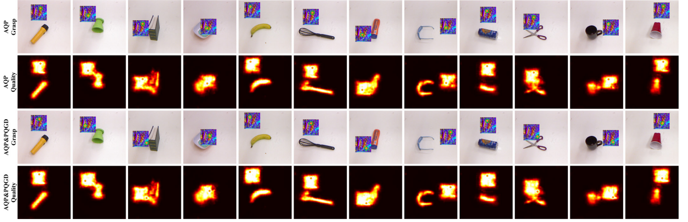
Fig. 5. Quality score visualization of AQP (first two rows) before and after adding PQGD (last two rows). Here, the GGCNN2 and the Cornell Grasp dataset are used to optimize the AQP. And AQP is scaled to 0.3 of the original size (the same size as the image).
