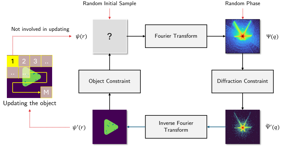
FIGURE 4.10: This illustration demonstrates the implementation of Skipped Region Strategy 2 within an iterative phase retrieval framework. The methodology employs selective regional exclusion during each iteration cycle, where a specifically designated area within the object domain (visually highlighted in yellow within the upper-left quadrant) is systematically omitted from update procedures through the application of a binary mask function M(x, y) . This designated region maintains its previous iteration values, effectively bypassing the phase retrieval feedback loop while preserving its original characteristics.
