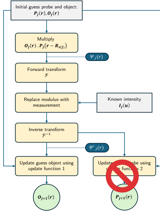
FIGURE 3.3: The customization of the ePIE algorithm of the Ptychography mechanism to single-frame CXDI.
