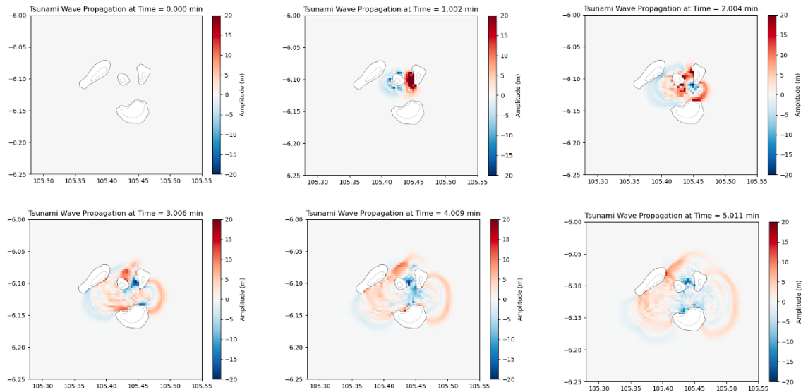
Figure 5.13 Snapshots of wavefield in 1–5 minutes in the east direction
