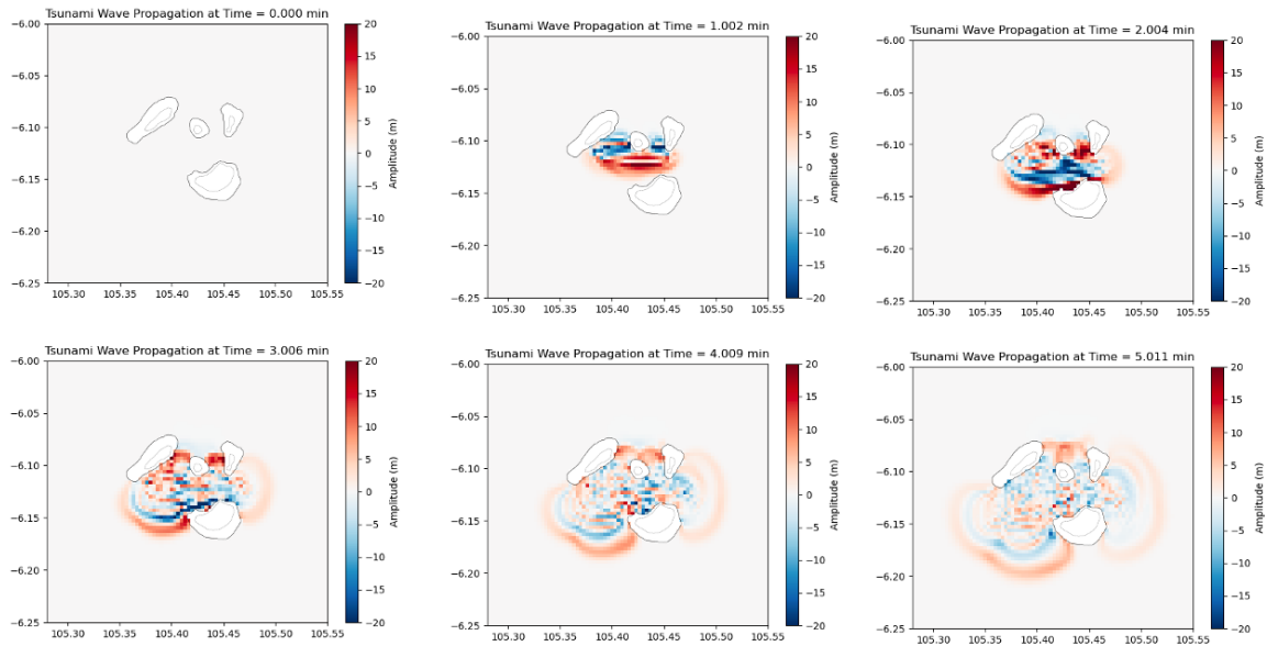
Figure 5.11 Snapshots of wavefield in 1–5 minutes in the south direction
