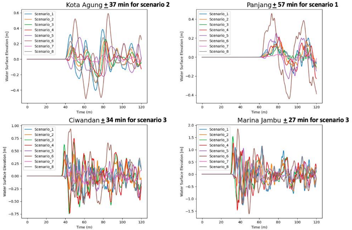
Figure 5.20 The first tsunami wave arrived within minutes recorded on tide gauges
