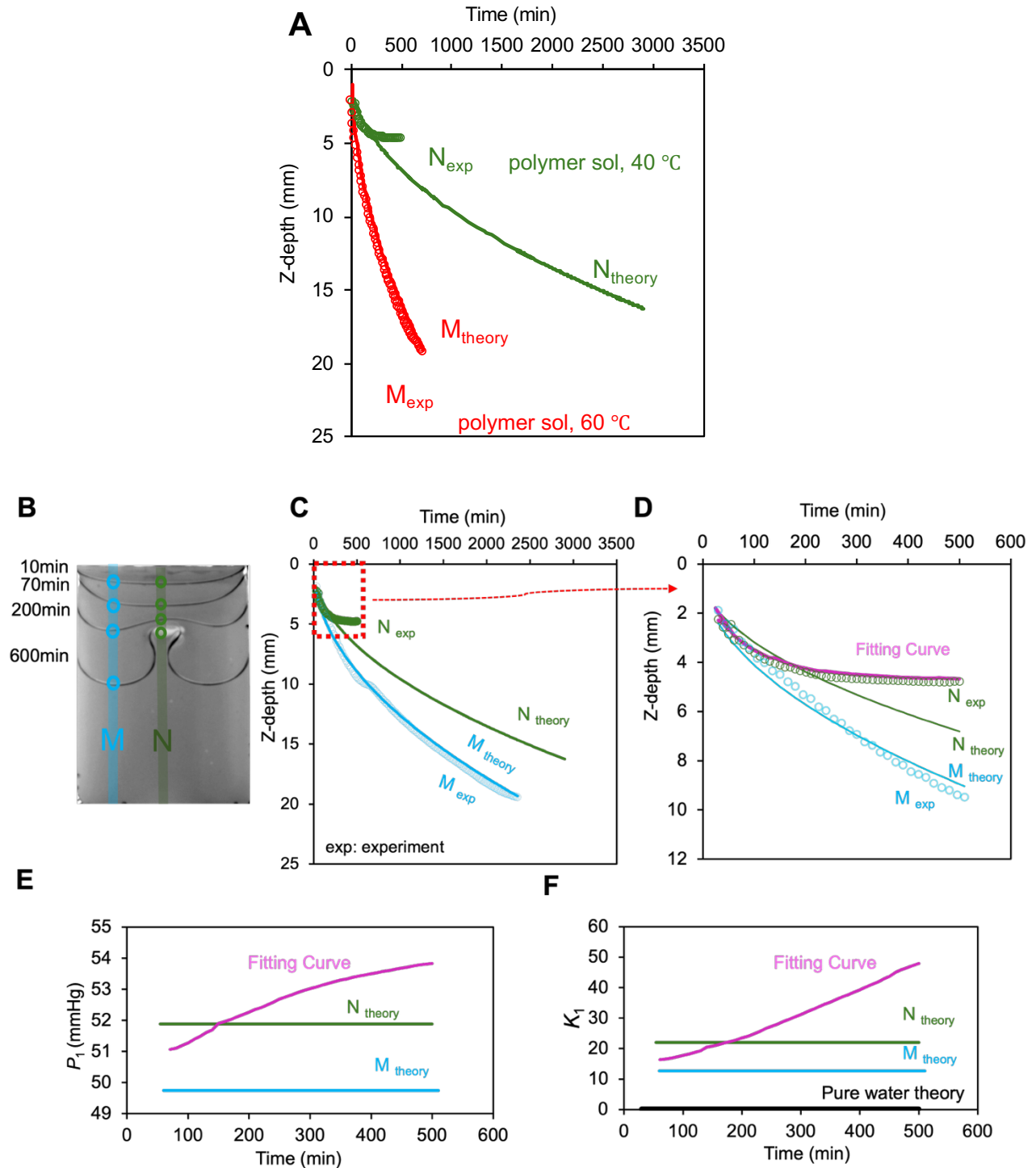
Figure 2.6. These theoretical/experimental curves of polymer solution at 40 and 60 °C (A), and comparison of interface positions at 40 °C (B, C, and D). Two important parameters affecting drying process at 40 °C (E, and F). Initial \lambda -carrageenan concentration: 1.5 wt.%. Cell dimensions: 15 mm \times 1 mm \times ~23 mm. The relative humidity was estimated to be 14.2 \pm 2.5\% RH.
