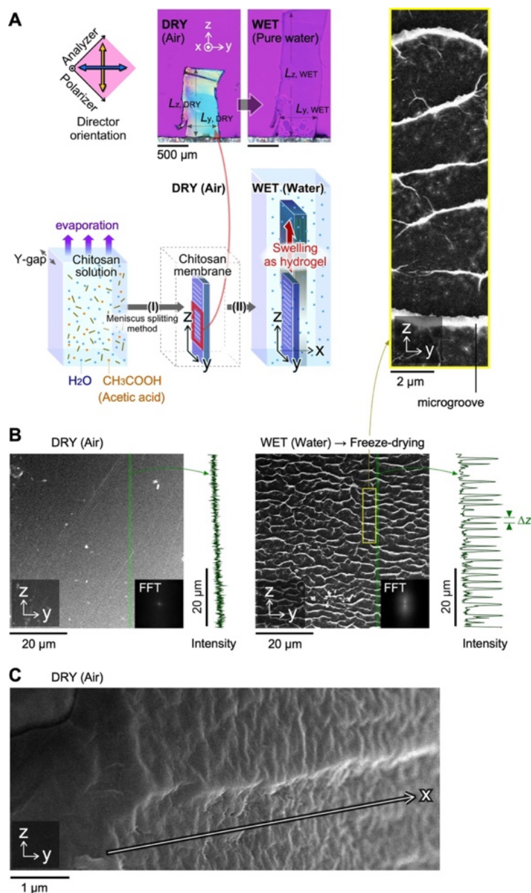
Figure 4.7. Chitosan hydrogel anisotropically swelling in pure water and its microstructures. A. Polarized optical microscopic images in air and in pure water. The process of the chitosan solution for the preparation of the DRY membrane and WET hydrogel. (I) Drying the aqueous chitosan solution includes acetic acid to form chitosan membrane using meniscus splitting. (II) Addition of pure water to the membrane. B. SEM images of the heat-dried sample prepared using the meniscus splitting method as DRY (air) and freeze-dried sample as WET (water). Inset: Fast Fourier Transformation (FFT) analytical data of SEM images. Charts indicate surface asperity on the YZ-plane of samples by analyzing the intensity of the gray value along the green line in the SEM images. Zoomed-in image in yellow-outlined area shows typical periodicity. C. SEM images of the heat-dried sample, focusing on the cross-section in the X-direction.
