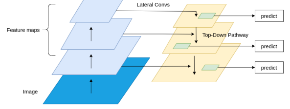
Fig. 5. Feature pyramid network structure
