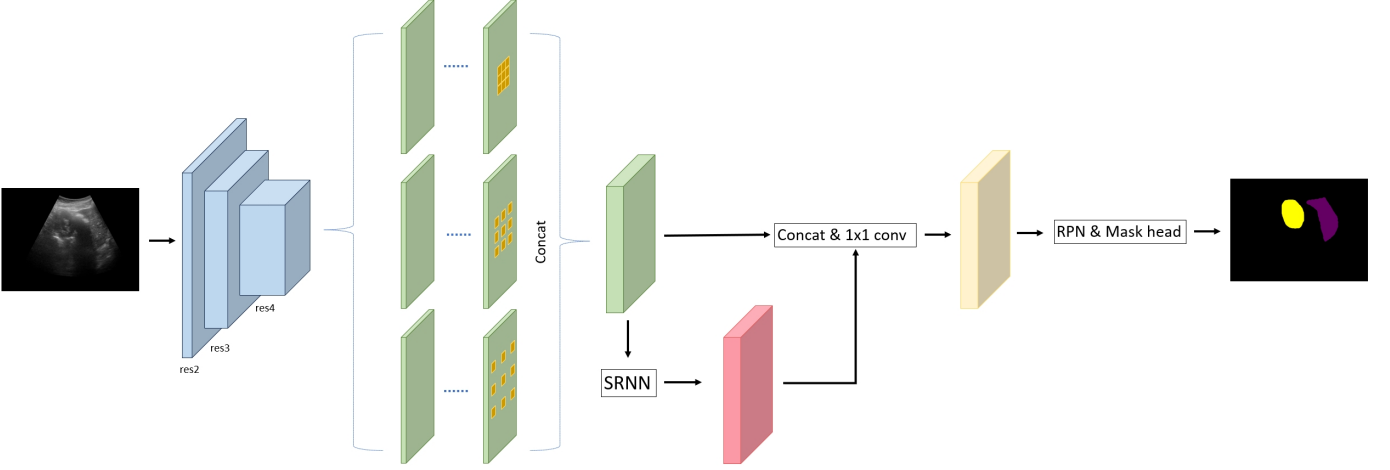
Fig. 9. Proposed network structure 2 based on trident network
