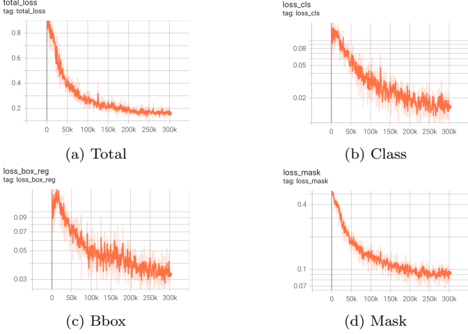
Fig. 12. Loss curves of FPN
