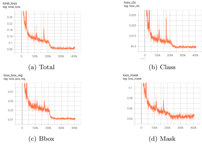
Fig. 13. Loss curves of Trident Network
