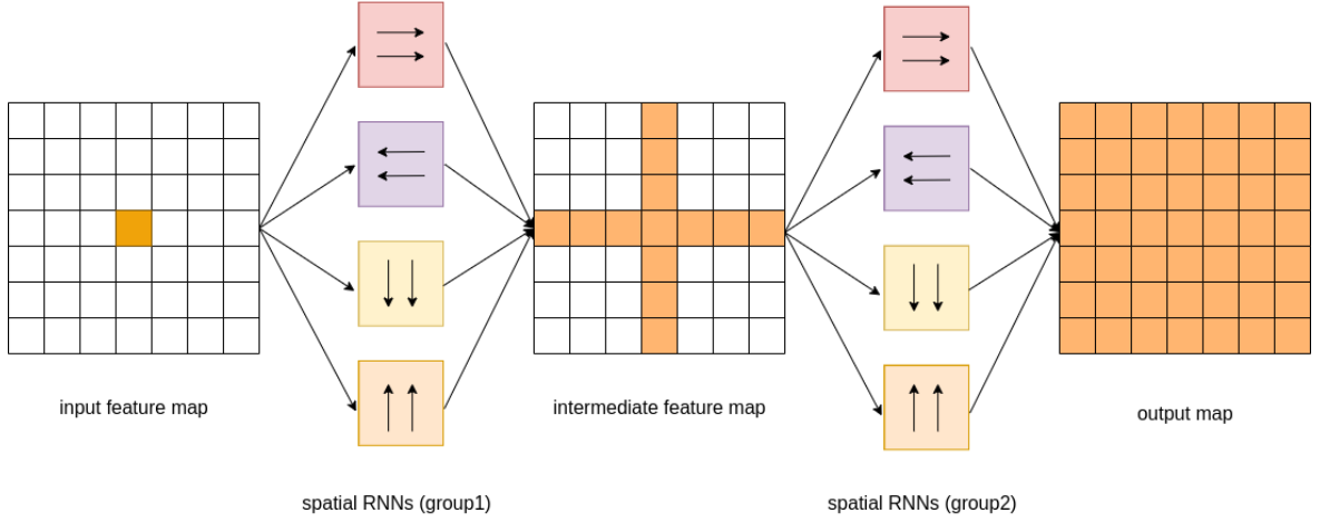
Fig. 10. Illustration of the IRNN propagation
