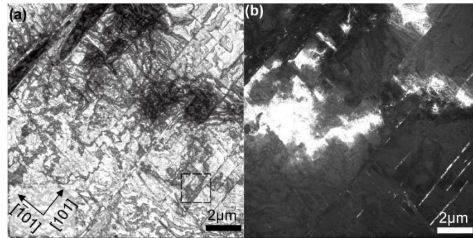
Figure 8. (a) BF- and (b) dark-field (DF)-TEM images of the No. 4 leaf. The DF-TEM image was taken by selecting the diffracted spot ( g = \bar{2}00 ). The bright narrow belts correspond to slip bands. Several bright narrow bands can be observed along not only the [101] direction but also the [\bar{1}01] direction. These bands are orthogonal with each other.
