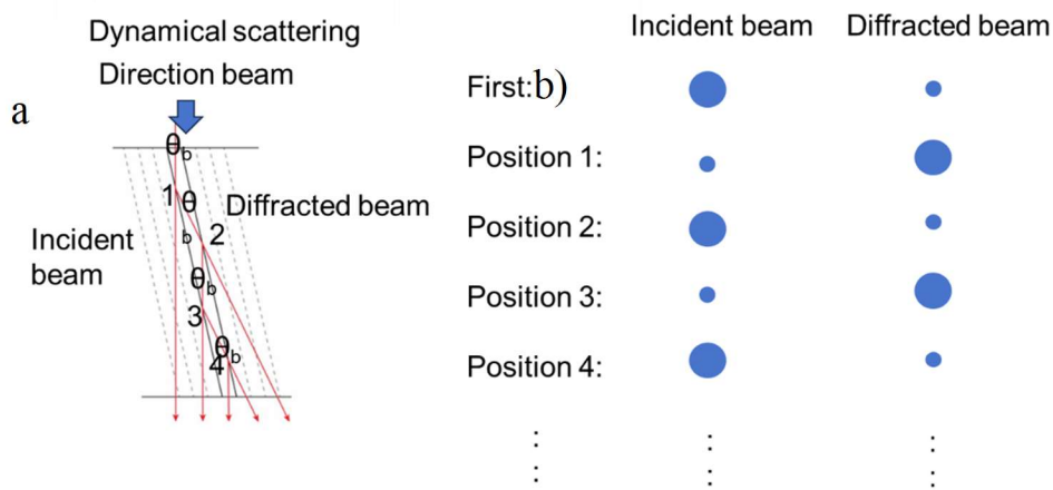
Figure 8. a) when direction beam passing through a crystal under an influence of the dynamical scattering; b) the relationship between the incident beam and diffracted beam after passing through several position which follow the Bragg law.
