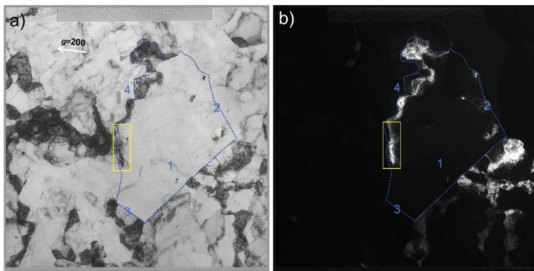
Figure 18. Ultra-high voltage TEM image of Al leaf form [001] direction. a) is the BF image; b) is the DF image.
