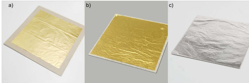
Figure 25. a) is the sheet of No.4 Kanazawa gold leaf with a thickness of 0.1\mu\text{m} ; b) is the sheet of Zumi gold foil with a thickness of 0.7\mu\text{m} ; c) is the sheet of Al leaf with a thickness of 0.37\mu\text{m} .
