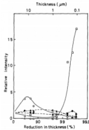
Figure 1. Variation of X-ray diffraction intensity of crystal planes as a function of thickness. The markers mean planes; \square (001), \circ (011), \blacktriangle (111), \triangle (012), \bullet (013) [3].
