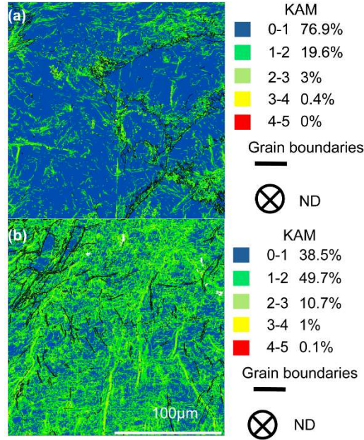
Figure 6. Kernel average misorientation (KAM) maps of the (a) Zumi foil and (b) No. 4 leaf. Colors indicate the average misorientation. Blue indicates a relatively small value, and green, yellow, and red indicate larger values in order. A larger value suggests the presence of a dislocation.
