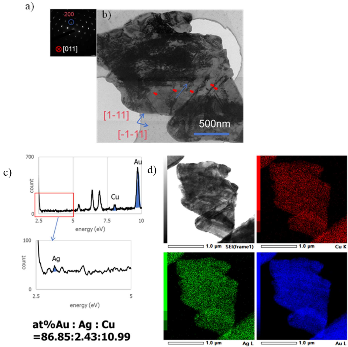
Figure 14. a) is the diffraction pattern form [011] direction; b) is the BF image form same condition; c) is eds spectrum analysis, showing the at% of every atom; d) is the eds elements map, red is for copper, green is for silver, blue is for gold.
