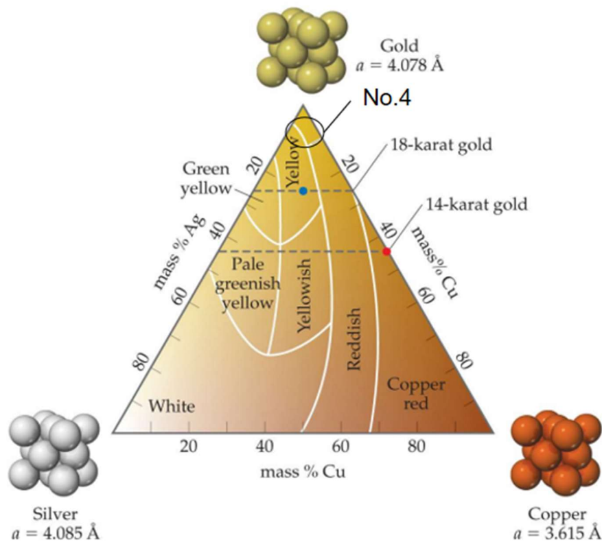
Figure 11 A ternary phase diagram of three elements Au, Ag, and Cu of color [6].
