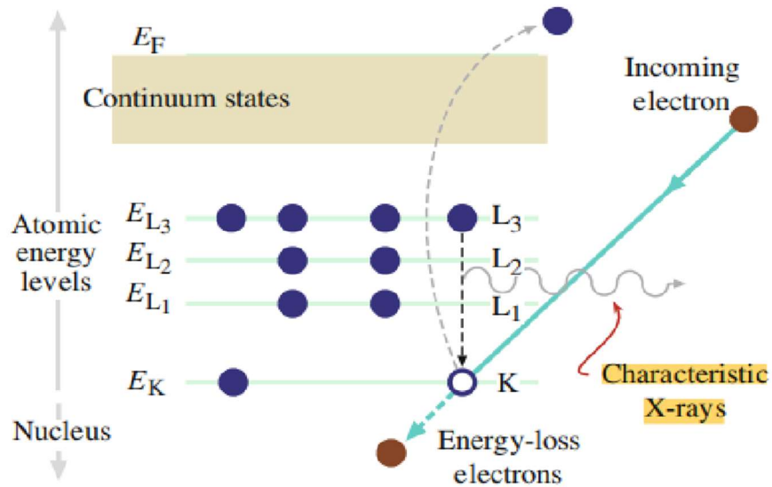
Figure14. Formation of Characteristic X-ray.
