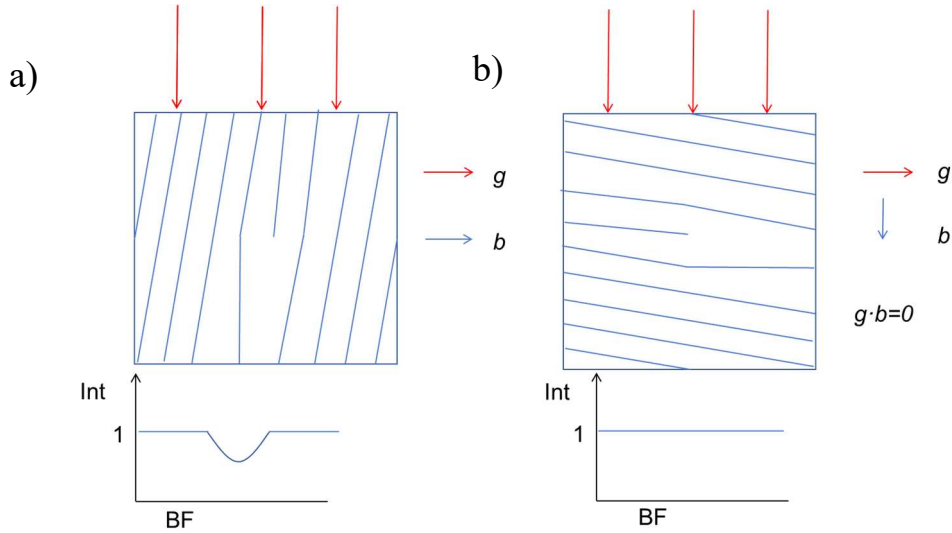
Figure 12. a) when the dislocation's Burgers' vector is not perpendicular with the diffraction vector b) when the Burgers' vector is perpendicular with the diffraction vector.
