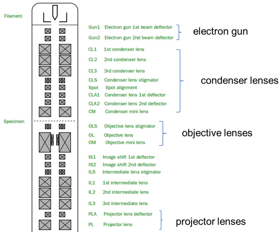
Figure 2. Main components of TEM[5].
