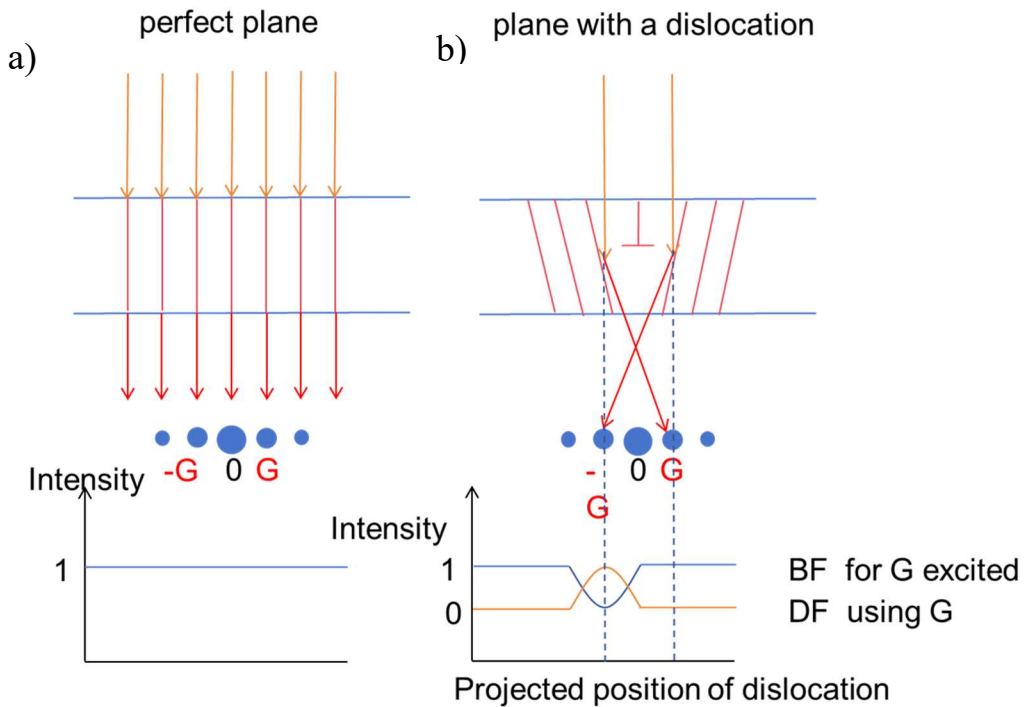
Figure 10. a) the beam passing by a crystal with perfect plane. (b): Intensity changes in BF and DF images due to the distorted planes.
