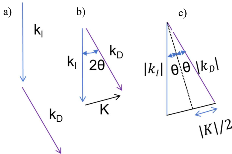
Figure 5. a) the incident wavefront normal is k_I , the diffracted wave normal is k_D ; (b) K is the difference vector; (c) \sin\theta is defined as K/2K_I [5].
