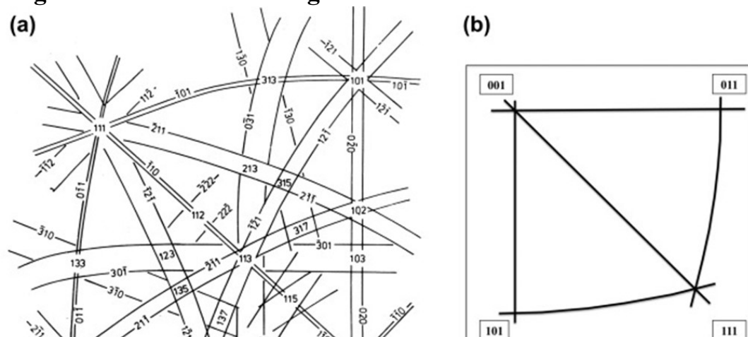
Figure 16. a) A Kikuchi map for FCC crystal (Taken from Loretto (1984)); b) The corresponding real-space stereogram. See text for explanation.
