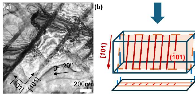
Figure 9. (a) BF-TEM image of the No. 4 leaf enlarged to show the local area shown in Fig. 5(a). A slip band with many dislocation lines arranged in a periodic pattern is formed along the [101] direction. (b) Schematic illustration of the slip plane and dislocations in the No. 4 leaf that can explain the slip band in (a). The blue arrow indicates the hammering direction (approximately [001] ). The slip plane was determined to be the (\bar{1}01) plane. The dislocations terminate at both surfaces with the Burger's vector of the [101] direction, which corresponds to screw dislocations. The dislocation lines are projected onto the screen.
