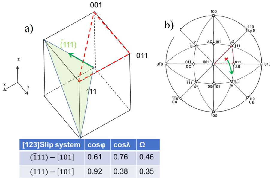
Figure 11.a) at the compress axis from [123] , the slip system shown in the green tangle will be start cause of the highest Schmid factor; b) as the slip system start the compress axis will rotate with the green arrow, to the [001] - [011] line.
