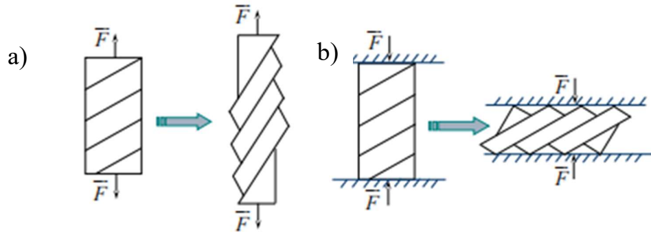
Figure 10.a) for stretching, the direction of slip seeks to turn (converge) towards the stretching axis; b) for compression, the slip surface tries to turn (converge) to the compression surface during slip surface.
