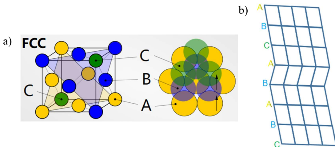
Figure 15.a) A, B, C marked with three types of color as three different types of \{111\} planes in FCC crystal; b) when one of the \{111\} planes change, such structure is so-called stacking fault.
