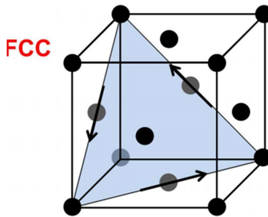
Figure 7. the blue triangle shows the \{111\} plane as the closest-packed planes and the arrow as the \langle 110 \rangle closest-packed direction.
