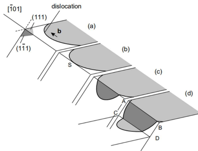
Figure 16. cross slip in the FCC metal.
