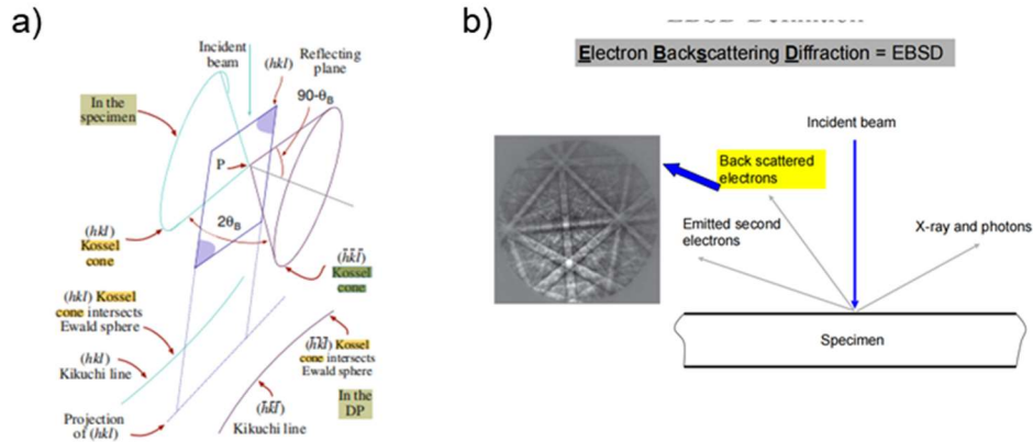
Figure 15. a) the formation of the Kossel cones and Kikuchi line. b) the EBSD base on SEM.
