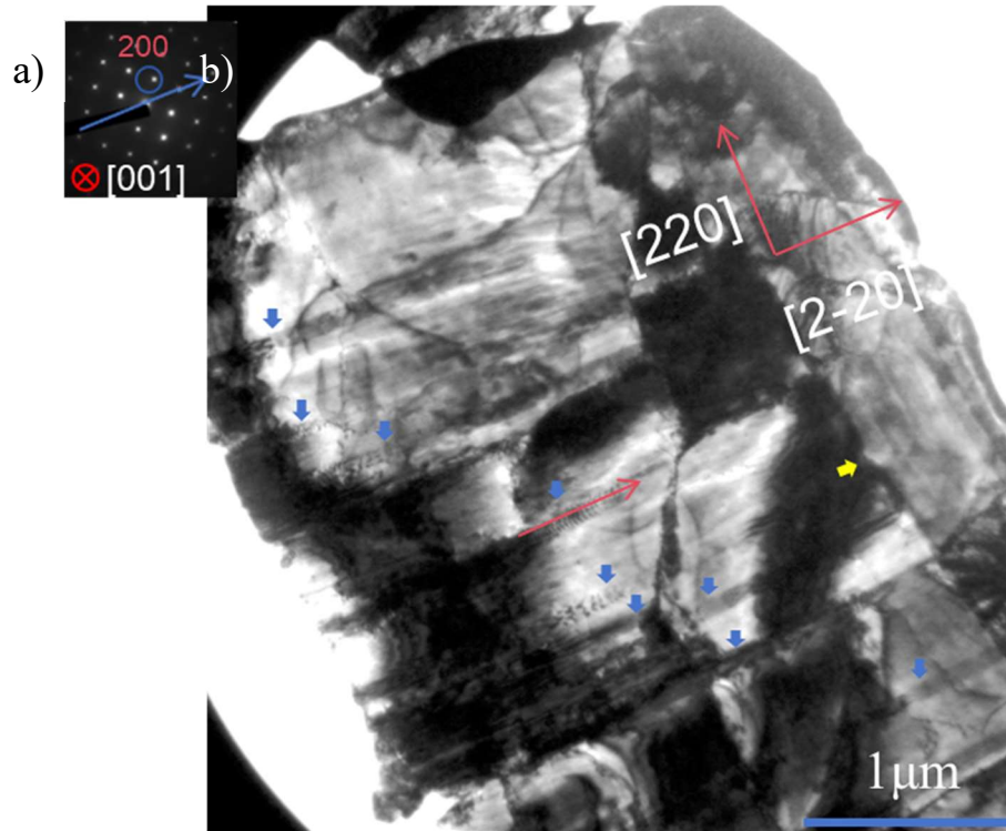
Figure 13. BF image form [001] direction for the No.4 gold leaf.
