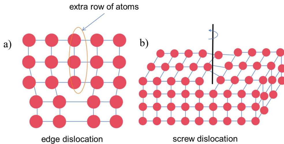
Figure 6. a) Edge dislocation b) Screw dislocation.
