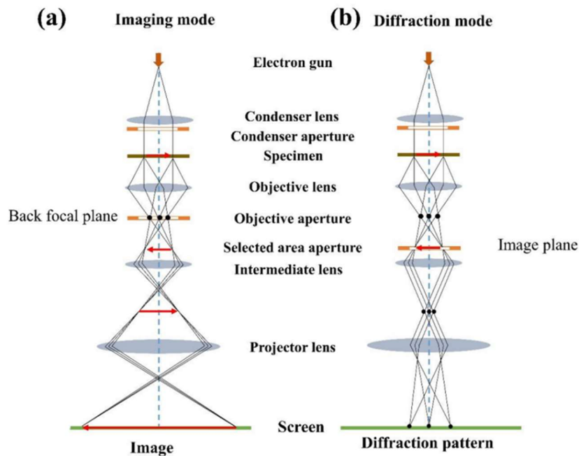
Figure 7.a) the image mode for TEM. b) the diffraction pattern mode for TEM, which is formed at or close to the back focal plane of the objective lens.
