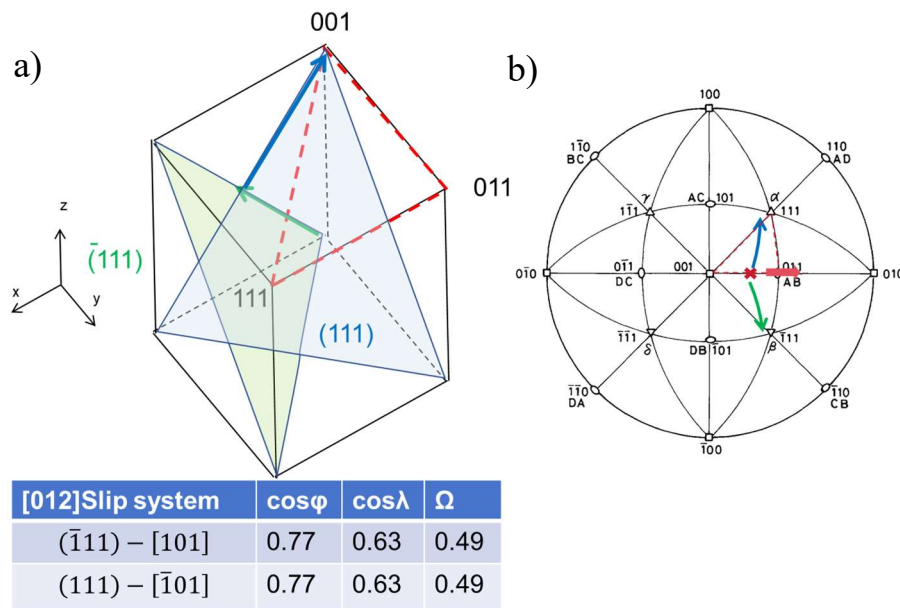
Figure12.a) at the compress axis from [012] , the slip systems shown in the green and blue tangles will be start cause of the highest Schmid factor; b) as the slip system start the compress axis will rotate with the red arrow which combining with the two arrow along the [001] - [011] line.
