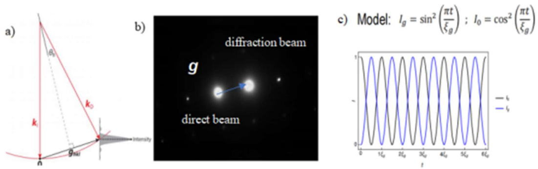
Figure 11. a) Two-beam condition with K_I and K_D following Bragg's Law; b) Diffraction pattern under the two-beam condition with a diffraction vector g ; c): Dynamic correlation between direct and diffracted beam intensities.
