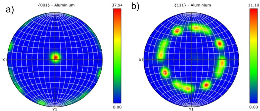
Figure 19. The pole figure form EBSD analysis. a) is the pole figure form \{001\} of the Al leaf; b) is the pole figure form \{111\} of the Al leaf.
