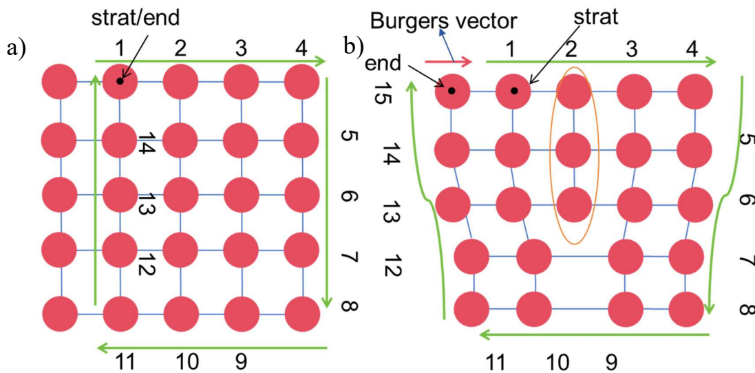
Figure 5. a) Perfect crystal b) When a dislocation in the crystal shows a burgers vector.
