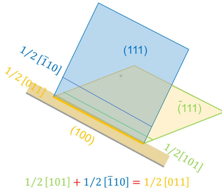
Figure 13. Dislocations from the secondary slip system can meet and interact. A so-called Lomer lock structure formatted at the edge of the planes.
