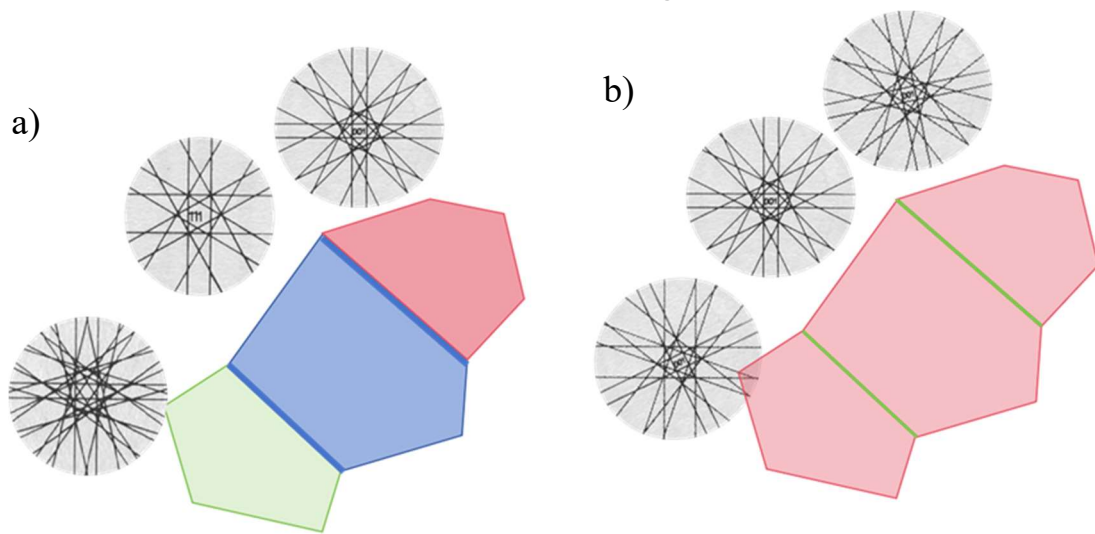
Figure 20 a) blue line is high angle grain boundary, green line is low angle grain boundary) between different crystals, there is a grain boundary which can detect by EBSD scanning. b) Even though some area only a little bit twist, EBSD can also identify how much angle differences are they.
