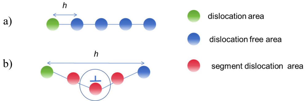
Figure 9.a) is the Perierls valley in a crystal with a low density of dislocation. b) is the Perierls valley in a crystal with a high density of dislocation, the h is much longer than it in a.
