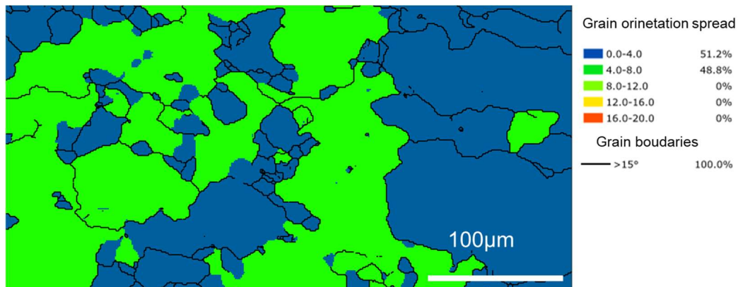
Figure 16. The GOS map, analysis from the HD.
