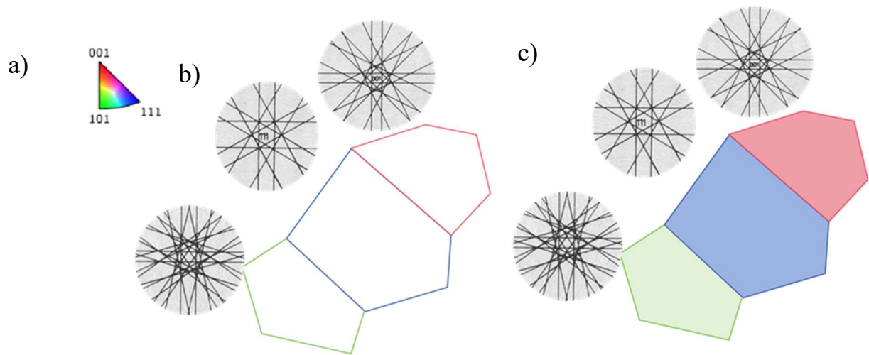
Figure 18. a) color scaling of IPF coloring; b) Kikuchi line which collect after EBSD scanning, which shows three types of different Kikuchi line of FCC from top is \{001\} , \{111\} , and \{011\} ; c) After IPF coloring, different crystals have a different color
