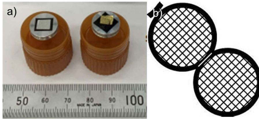
Figure 26. a) shows the Al leaf and gold leaf secured on the sample stage; b) is the double grid used for the sheet sample to make the TEM sample.
