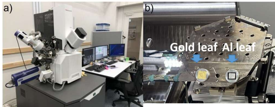
Figure 29. a) is ThermoFisher Scios2 dual-beam SEM with an Oxford Instruments EDS detector; b) shows the samples during the testing.
