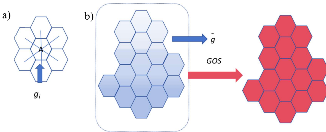
Figure 22. a) detect the orientation data for a single pixel. b) every \bar{g} in the whole crystals for each pixel) GOS color for every points.
