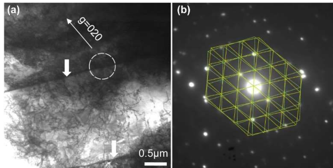
Figure 7. (a) Two-beam bright-field (BF)-TEM images of the Zumi foil under the condition g = 020 . (b) Local diffraction pattern for the dashed white circle in (a).
