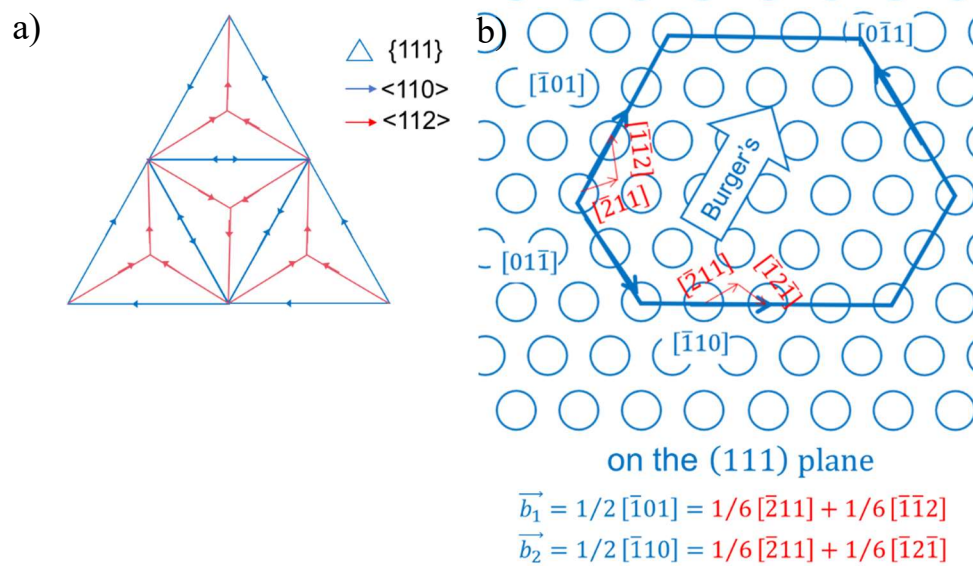
Figure 14.a) Shows possible slip directions within the \{111\} plane. The arrows represent different dislocation paths, with blue arrow for perfect dislocations and the red arrow for the partial dislocation; b) Shows the hexagonal close-packed arrangement of atoms on the \{111\} plane. The blue arrow labeled "Burgers" shows the Burgers vector ( \vec{b} ). The dislocations can decompose into partial dislocations, as indicated by the equations, which show how perfect dislocations break into partials.
