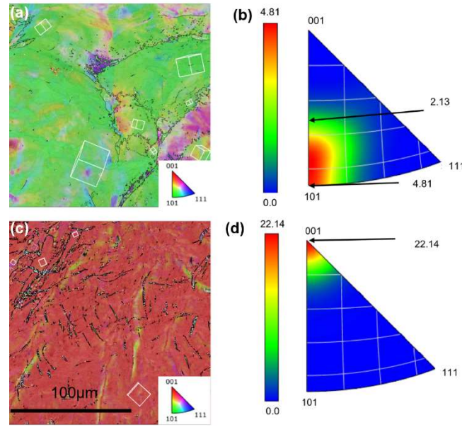
Figure 4. Inverse pole figure (IPF) coloring maps of the (a) Zumi foil and (c) No. 4 leaf. The color scale is derived from orientations aligned perpendicular to the sample surface (red, green, and purple correspond to the {001}, {110}, and {111} planes, respectively; black curves correspond to grain boundaries with misalignment angles greater than 15^\circ ; white lines depict the projected unit cell of the cubic structure). IPFs from the Z-axis of the (b) Zumi foil and (d) No. 4 leaf.
