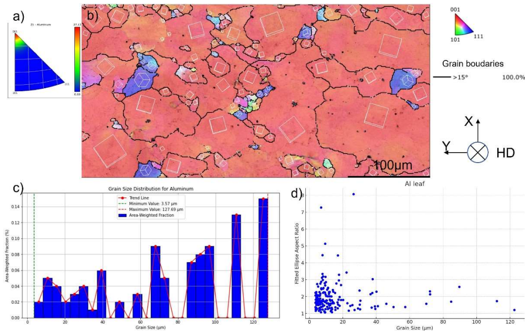
Figure 15. the EBSD data for Al leaf from HD. a) is the IPF figure; b) is the IPF-color map; c) is the grain size in such area; d) is the aspect ratios combine with the grain size.
