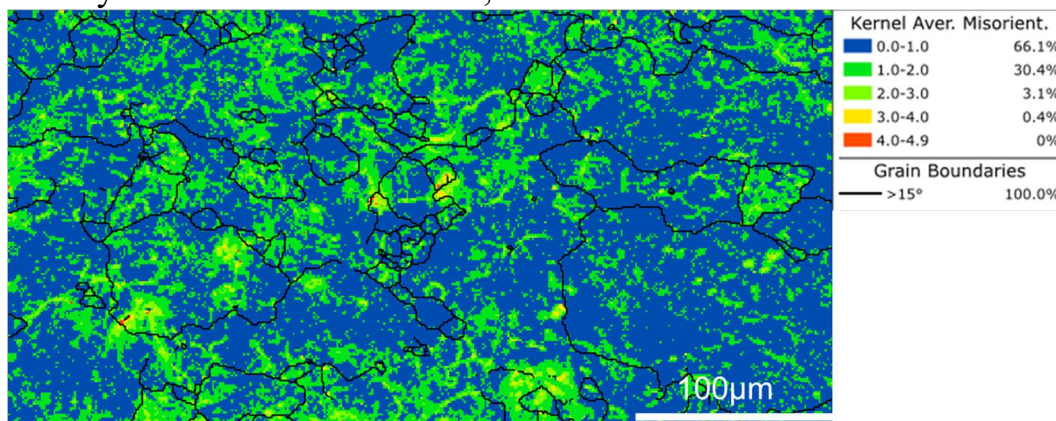
Figure 17. The KAM map analysis from the HD.
