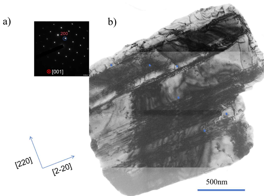
Figure 12. BF field image from [001] direction from pure gold leaf.
