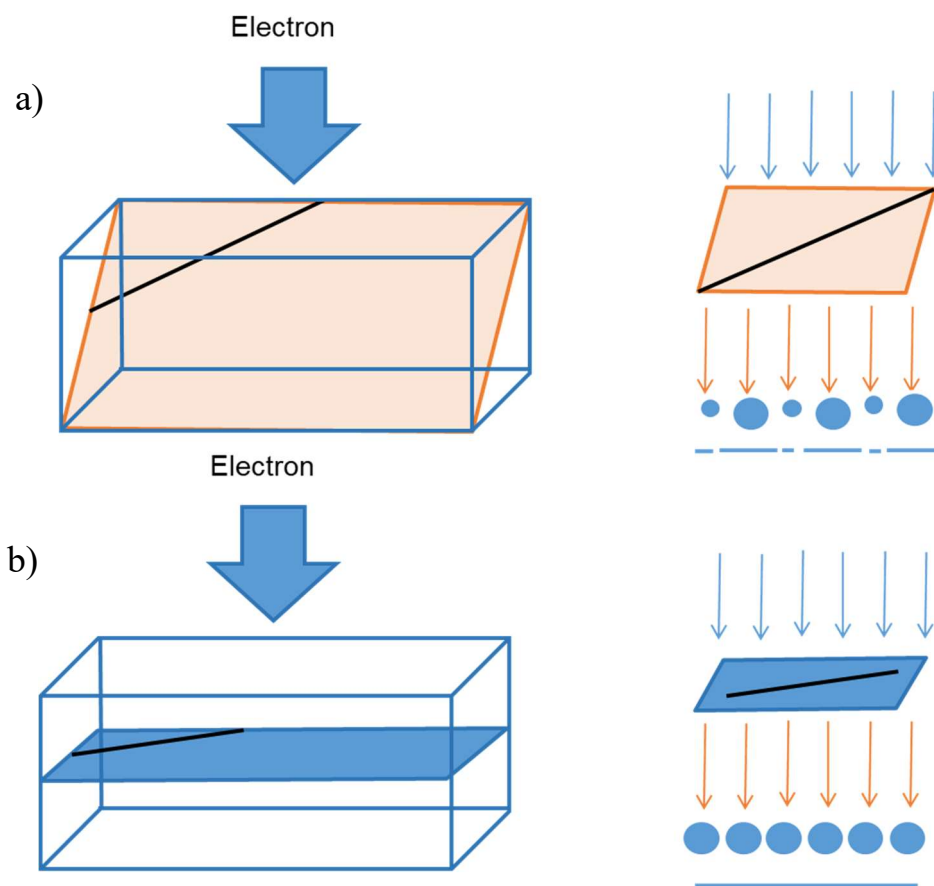
Figure 13.a) when a dislocation lies on planes non-perpendicular to the incident electron beam; b) lies on planes perpendicular to the incident electron beam
