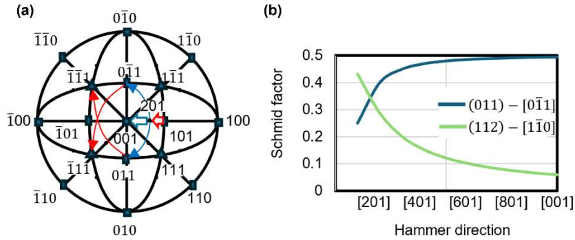
Figure 10. (a) Standard stereographic projection of the FCC crystal structure viewed from the [001] direction. After formation of the (101) texture, the hammering direction gradually changed from the [101] to the [201] direction by activation of either the (\bar{1}\bar{1}1)-[011] or (\bar{1}\bar{1}1)-[0\bar{1}1] slip system (red curves). It gradually changed from the [201] to the [001] direction by activation of either the (0\bar{1}1)-[011] or (011)-[0\bar{1}1] slip system (blue curves). These slip systems are non-octahedral. (b) Schmid factors for non-octahedral slip systems as a function of the hammering direction. The Schmid factor of the (112)-[1\bar{1}0] slip system was high when the hammering direction was approximately along the [101] direction. However, the Schmid factor of the (011)-[0\bar{1}1] slip system increased when the hammering direction changed from the [201] to the [001] direction.
