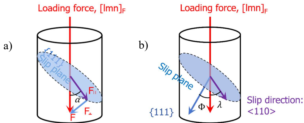
Figure 8. the relationship between slip plane, slip direction and loading force of a) shows the shear force; b) shows the Schmid factor.
