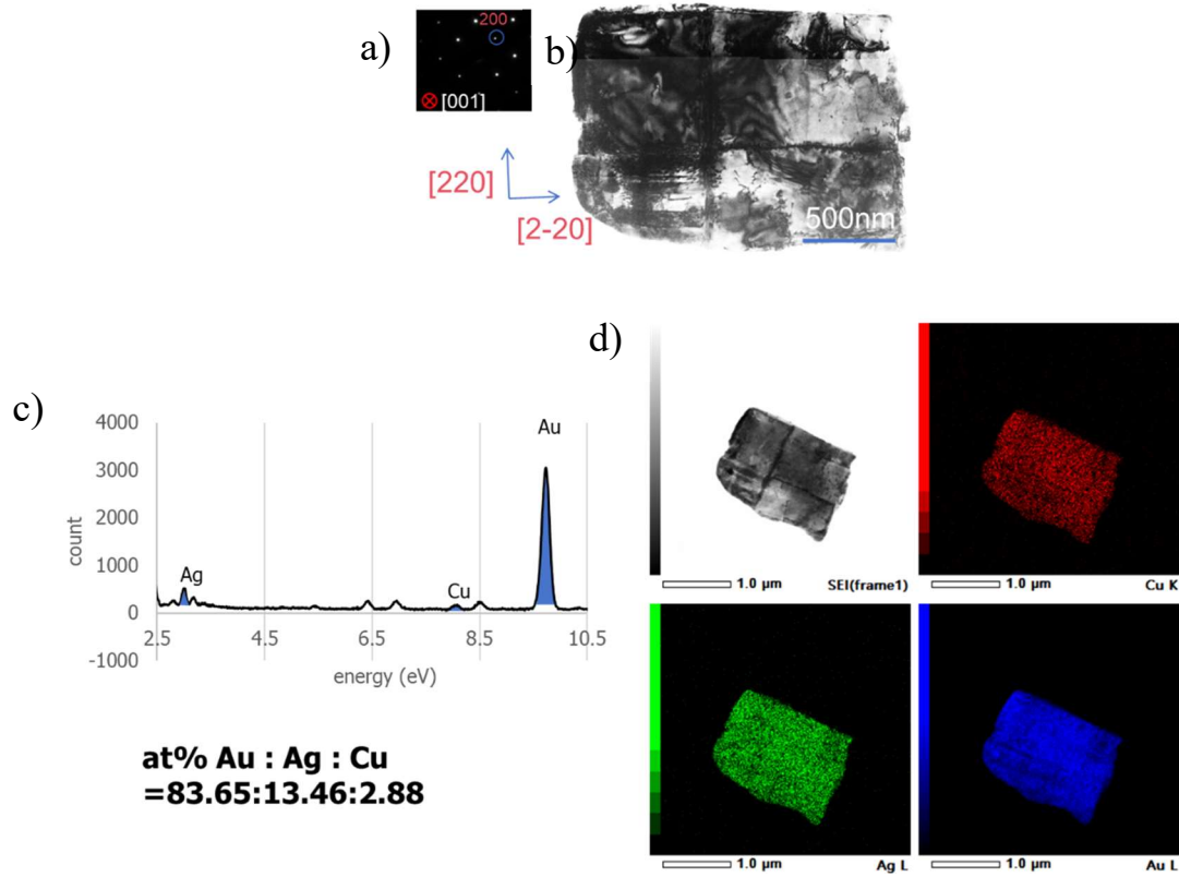
Figure4. a) is the diffraction pattern form [001] direction; b) is the BF image form same condition; c) is eds spectrum analysis, showing the at% of every atom; d) is the eds elements map, red is for copper, green is for silver, blue is for gold.
