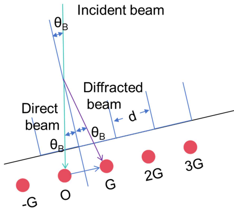
Figure 6. Diffraction spots formed when an incident beam passes through the crystal [5].
