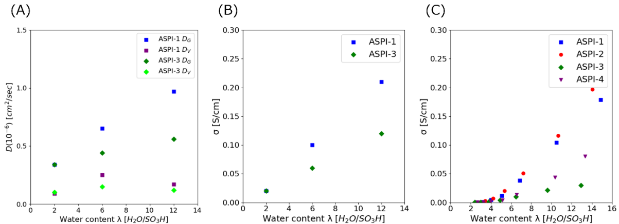
Figure 5. The diffusion coefficient ( D ) and proton conductivity ( \sigma ) in the function of water uptake ( \lambda ) for ASPI-1 and -3 from computational simulations (A, B) and experimental investigations 7 (C).
