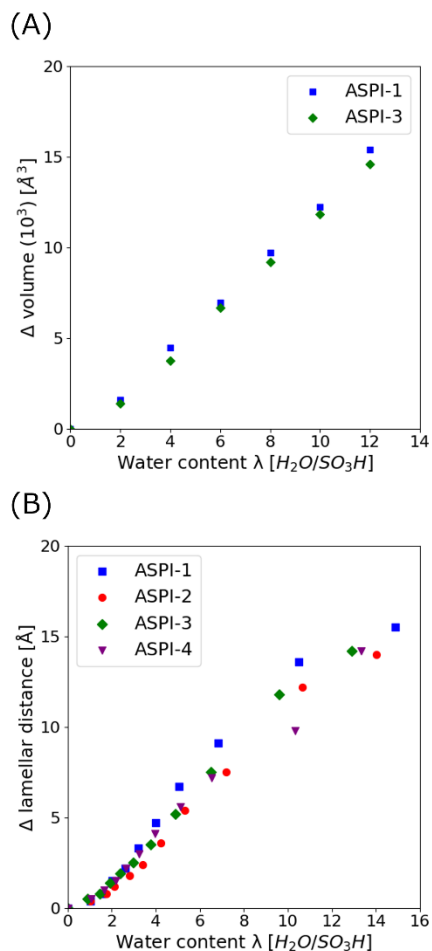
Figure 4. Change of the volume and lamellar distance in function of hydration level ( \lambda ) from computational simulations (A) and experimental investigations 7 (B).
