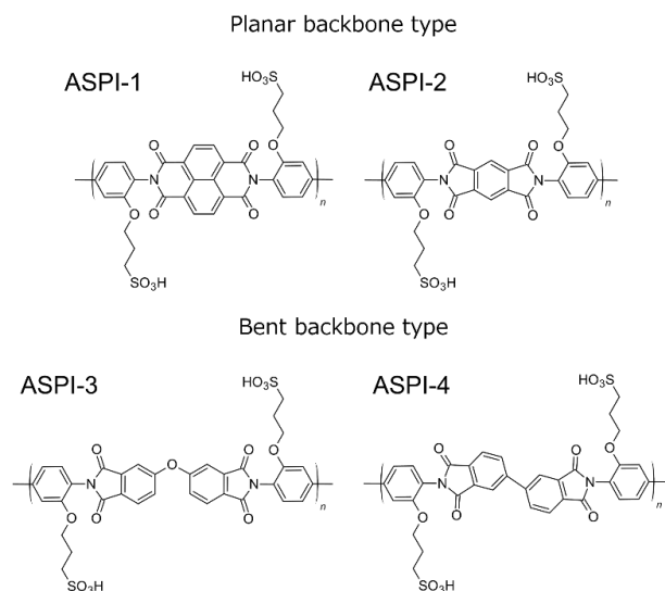
Figure 1. Chemical structures of planar (ASPI-1 and ASPI-2) and bent (ASPI-3 and ASPI-4) backbone ASPIs.
