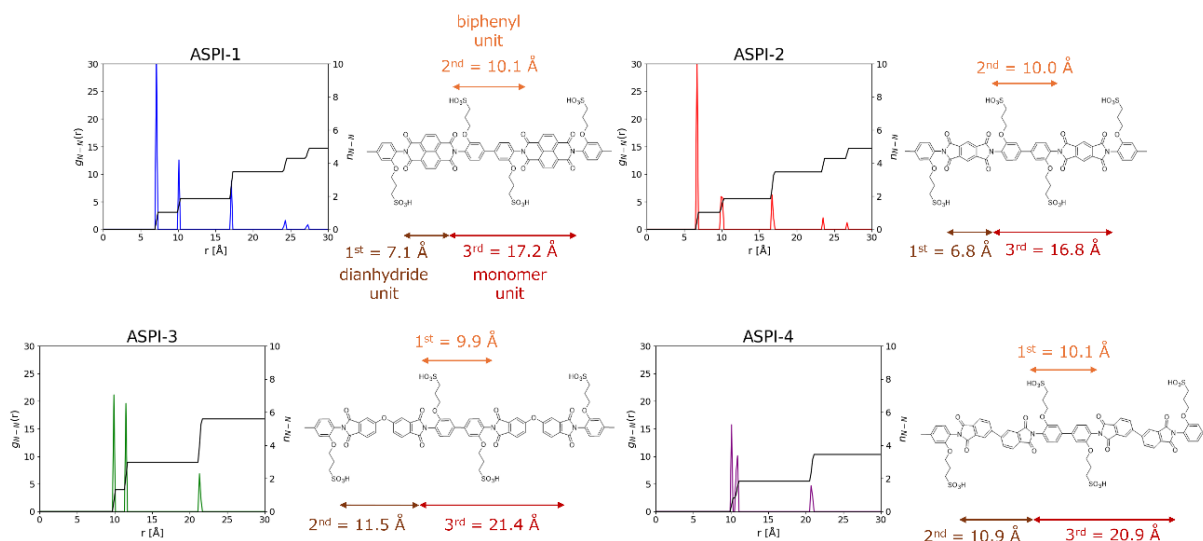
Figure 2. The N–N RDF for the single polymer chains (n = 5) of ASPIs to define the key units within the single polymer chain.
