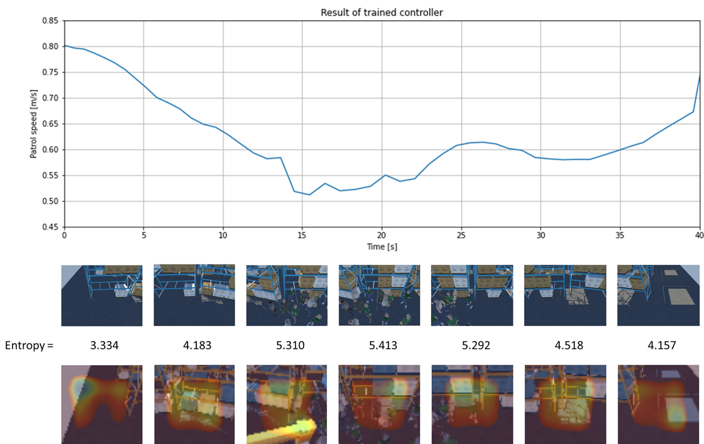
Figure 14 Simulation results of the trained patrol speed controller. (Top) input images and corresponding speeds at seven locations. (Bottom) Grad-CAM visualizations.
