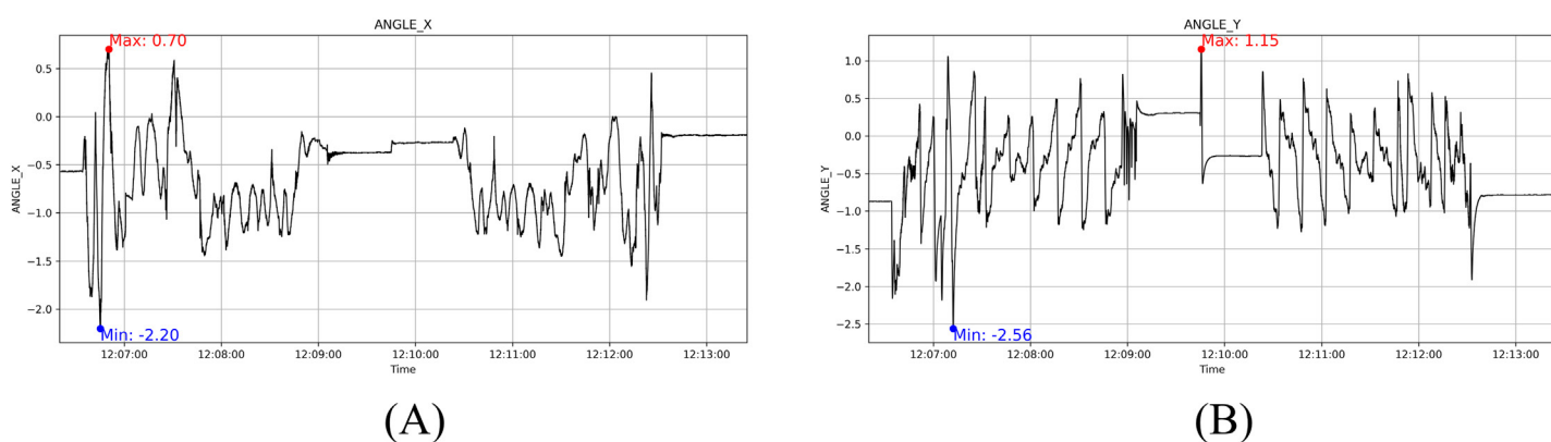
Figure 15 Rail inclination measurement results during constant-speed driving. (A) Roll angle (ANGLE_X). (B) Pitch angle (ANGLE_Y).
