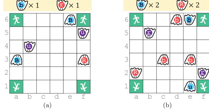
Figure A.14: Examples of pruning heuristics for (a) escape and (b) capture.
