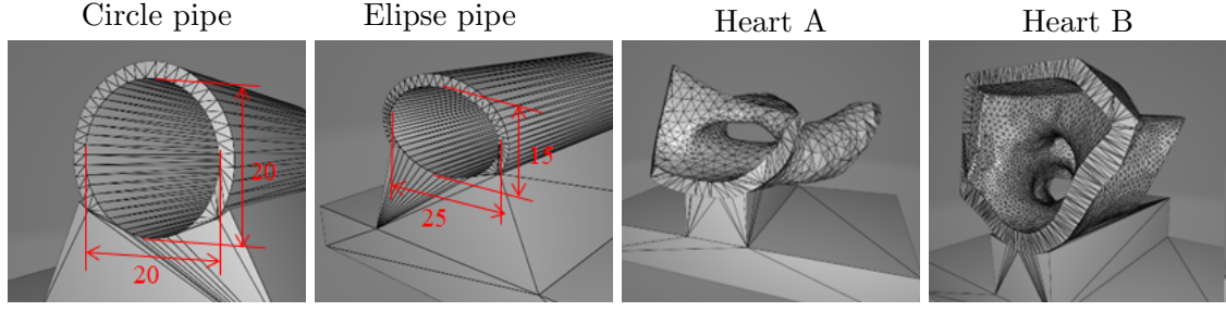
Fig. 4.7: Contact targets for contact area estimation. 3D shapes used for contact estimation evaluation.
