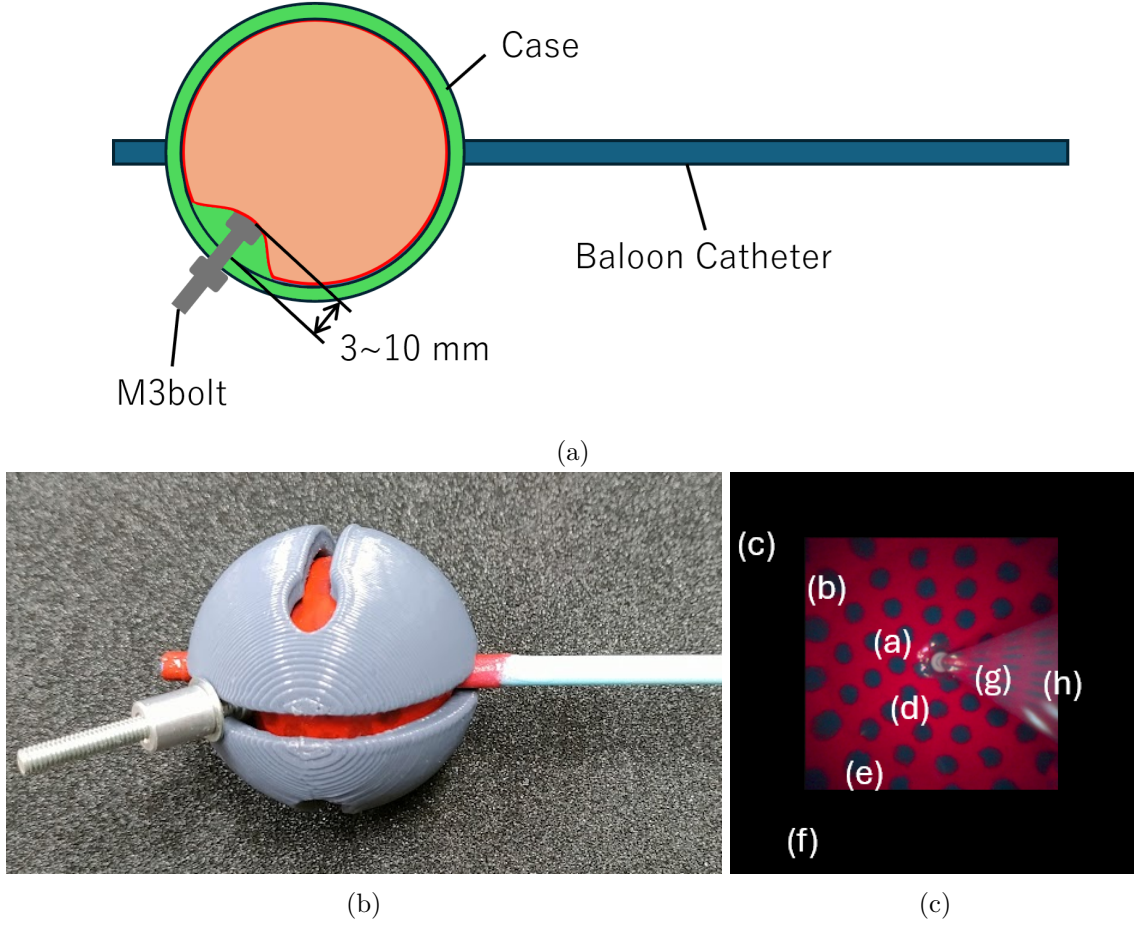
Fig. 4.1: Experimental design of the depth evaluation experiment. (a) Schematic of the experiment: the tactile balloon catheter is inserted into the inner cavity of the case and inflated. An M3 bolt mounted on the case is advanced to impose a prescribed indentation depth on the balloon surface. (b) Photograph of the actual experimental setup. (c) Contact positions: each contact point has the following characteristics: (a, b, d, e, g) positions within the camera field of view; (c, f, h) positions outside the field of view; (g, h) positions that are partially occluded by the inner tube.
