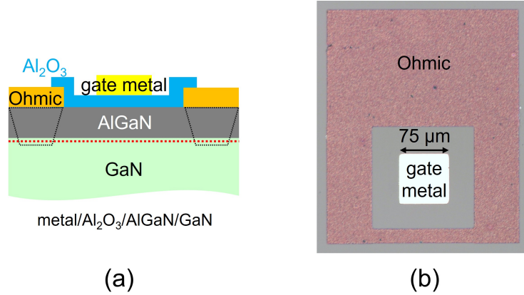
FIG. 1: (a)The schematic and (b)the top view of the metal/ \text{Al}_2\text{O}_3 /AlGaN/GaN capacitor devices.
