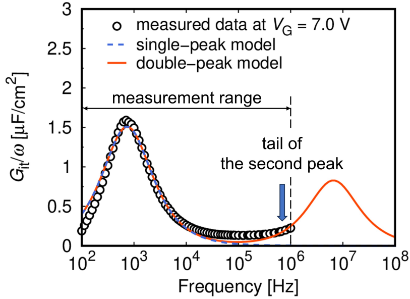
FIG. 10: Measured G_{\text{it}}/\omega in comparison with calculated curves obtained by the single- and double-peak models.
