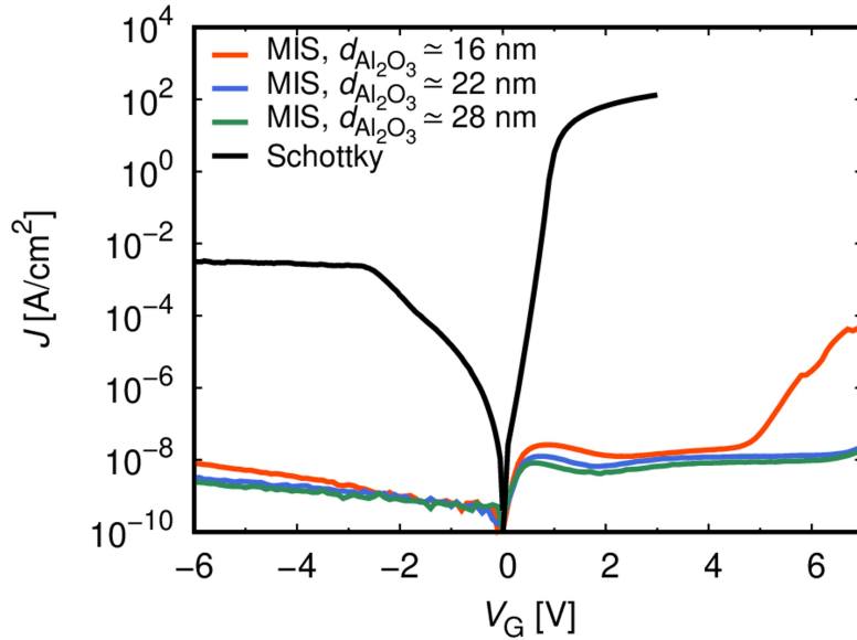
FIG. 2: J - V characteristics of metal/ \text{Al}_2\text{O}_3 /AlGaIn/GaN MIS devices, in comparison with that of a metal/AlGaIn/GaN Schottky device.
