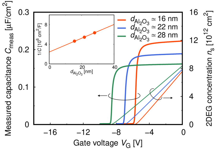
FIG. 3: C - V and n_s - V characteristics of the metal/ \text{Al}_2\text{O}_3 / \text{AlGaIn} / \text{GaN} MIS devices. Inset: 1/C as a function of d_{\text{Al}_2\text{O}_3} .
