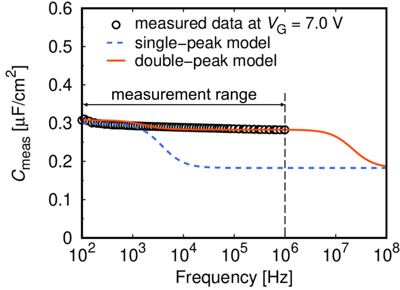
FIG. 11: Measured capacitance C_{\text{meas}} in comparison with calculated curves obtained by the single- and double-peak models.
