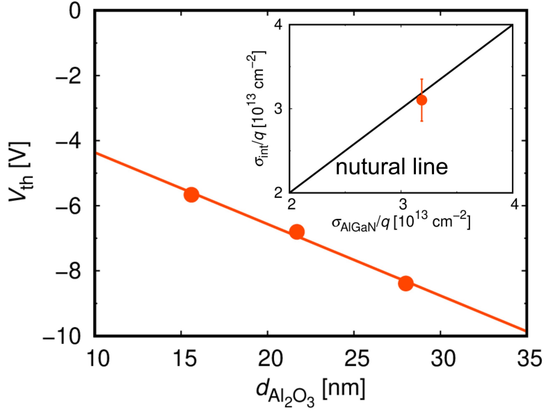
FIG. 4: The threshold voltages V_{\text{th}} as a function of d_{\text{Al}_2\text{O}_3} . Inset: the interface fixed charge density \sigma_{\text{int}} in comparison with the \text{AlGaIn} polarization charge density.
