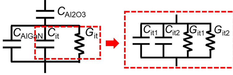
FIG. 7: The equivalent circuit for the double-peak model [44–47].
