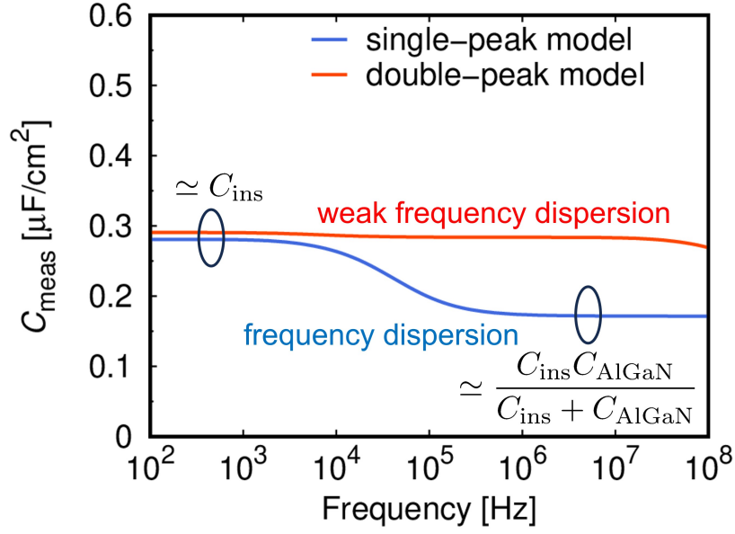
FIG. 9: The calculated prediction of the measured capacitance C_{\text{meas}} as functions of frequency based on the single- and double-peak models.
