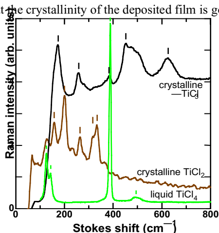
Fig. 1: Raman spectra of \text{TiCl}_n ( n=2, 3, 4 )
