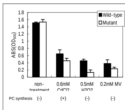
Figure 3. Enhancement of \text{Cd}^{2+} , \text{H}_2\text{O}_2 and methyl viologen (MV) tolerance to E. coli , and PC synthesis.
