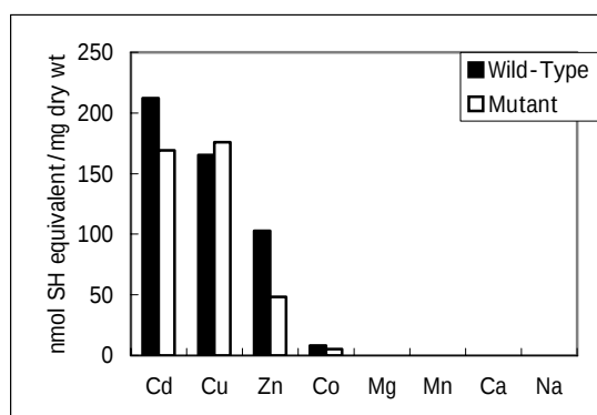
Figure 4. HPLC profiles of the interaction between wild-type and mutant PC synthase and metal ions. 0.5mM CdCl_2 , CuCl_2 , ZnCl_2 , CoCl_2 , MgCl_2 , MnCl_2 , CaCl_2 or NaCl was used for the analysis.
