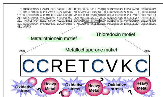
Figure 2. Amino acid sequence of the PC synthase and hypothetical model for PC synthase regulation
