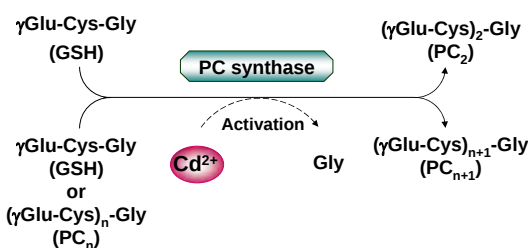
Figure 1. PC synthase catalyses the synthesis of PCs, (\gamma\text{Glu-Cys})_n\text{-X} polymers, by the net transfer of a \gamma\text{Glu-Cys} unit from one thiol peptide (usually GSH) to another, or to a previously synthesized PC molecule.
