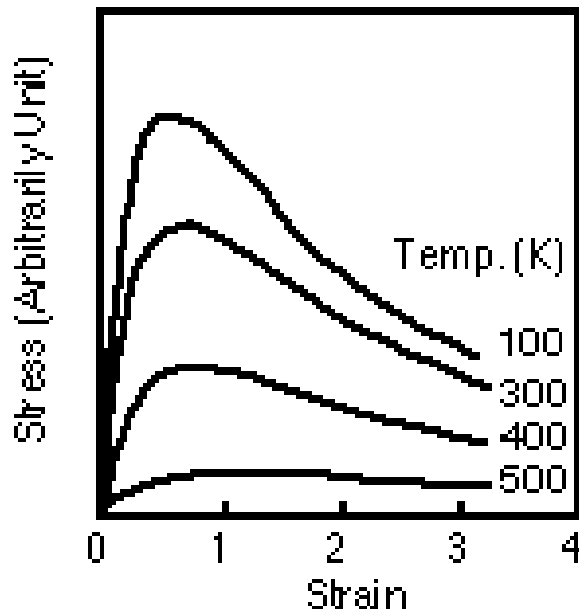
図 2: Temperature dependence of theoretical S-S curves
