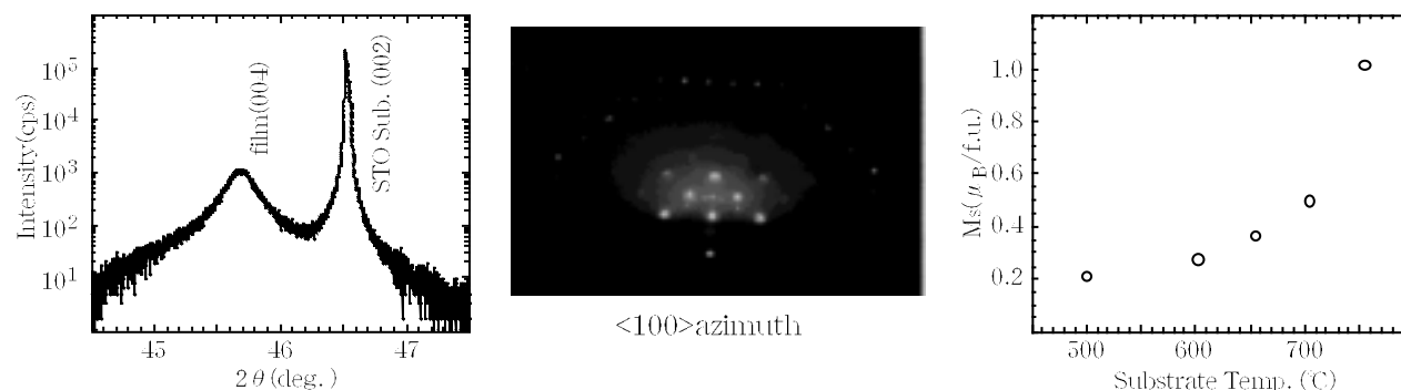
図 1: X-ray diffraction diagram of \text{Sr}_2\text{FeMoO}_6 film grown at 600 °C. 図 2: RHEED image of a \text{Sr}_2\text{FeMoO}_6 film grown at 600 °C. 図 3: Saturation magnetization of \text{Sr}_2\text{FeMoO}_6 films measured at 5K.
