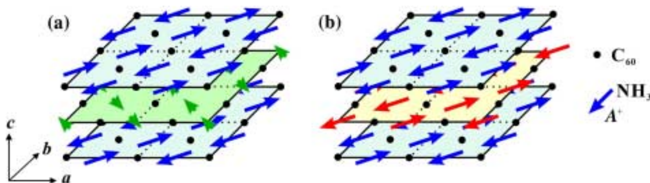
Fig. 構造モデル (a) (\text{NH}_3)\text{K}_3\text{C}_{60} , (\text{NH}_3)\text{K}_2\text{RbC}_{60} , (\text{NH}_3)\text{KRb}_2\text{C}_{60} (b) (\text{NH}_3)\text{Rb}_3\text{C}_{60}
