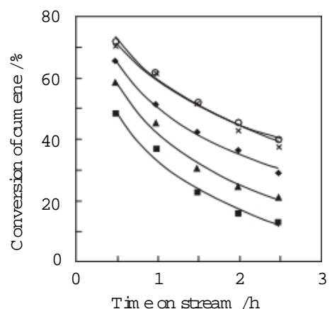
Fig.2 Conversion profiles of cumene on various A1SBA-15 samples.
