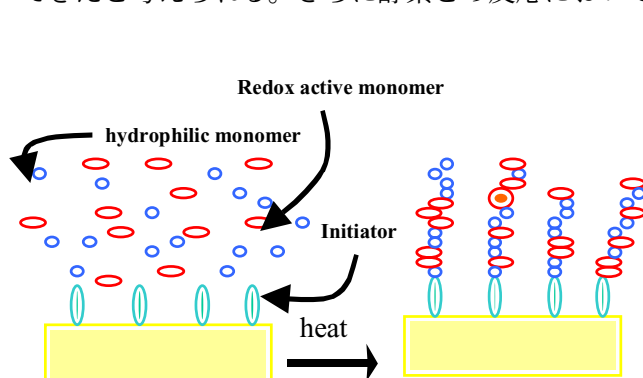
Fig. 1 Surface polymerization
