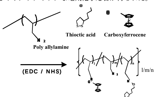
Fig. 2 Redox active polymer containing disulfide
