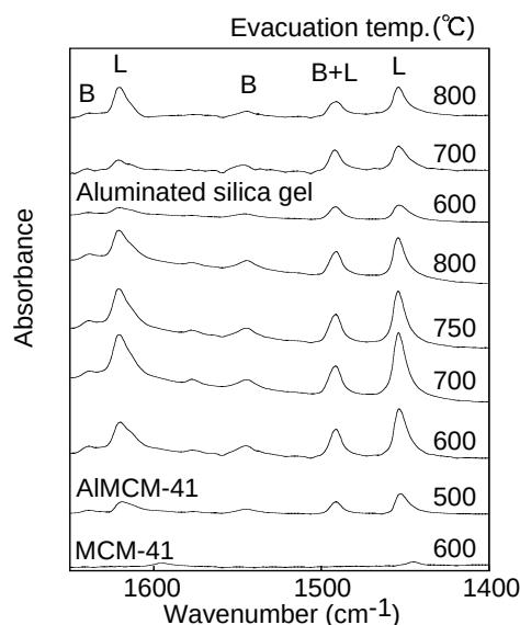
Figure 1 FTIR spectra of pyridine adsorbed on AIMCM-41 and MCM-41 evacuated at various temperatures.
