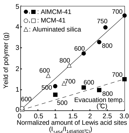
Figure 2 Relationship between normalized amount of Lewis acid sites and yield of polymer.
