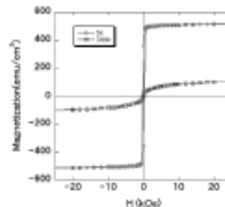
Fig. 3 Magnetic hysteresis loops
