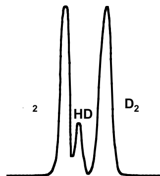
Fig.3 \text{H}_2 - \text{D}_2 exchange reaction (pretreatment time: 0.31s)
