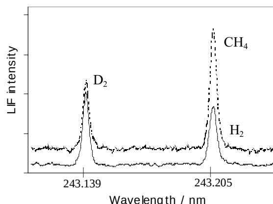
Fig.1 Two photon LIF spectra in H_2/D_2 and CH_4/D_2 systems
