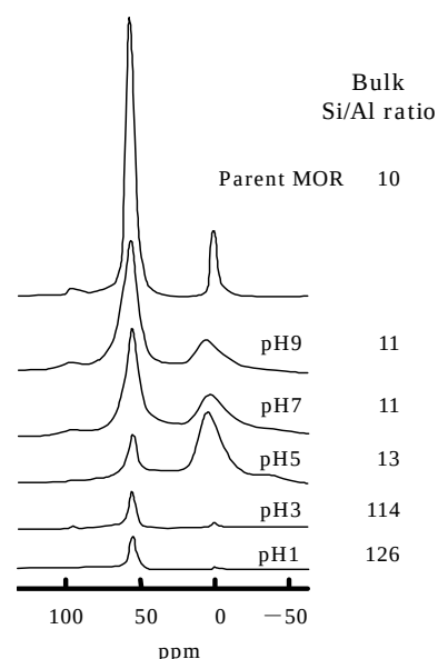
Fig.1 27 Al MAS NMR spectra of various MOR zeolite samples
