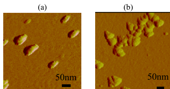
Figure 1 AFM images of (a) after heat treatment and (b) after TEA modification
