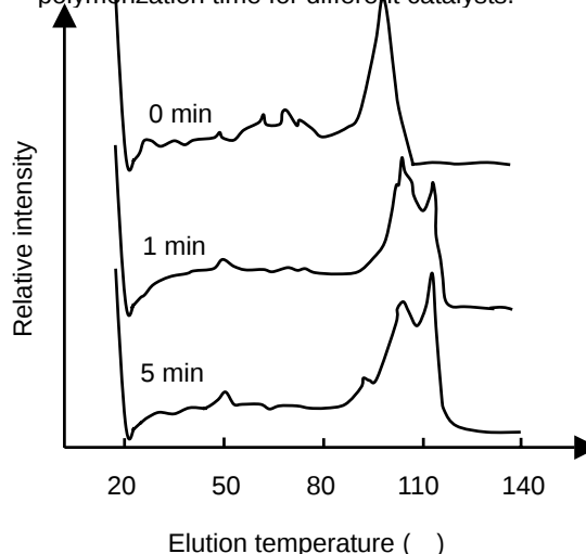
Figure 2 Dependence of TREF profiles on reaction time between catalysts and co-catalysts for PPs synthesized using Cat. A.
