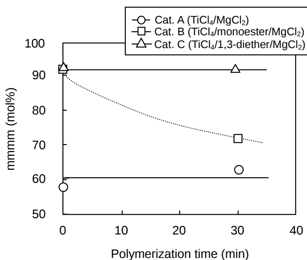
Figure 1 Isotacticity of resulting polymers versus polymerization time for different catalysts.
