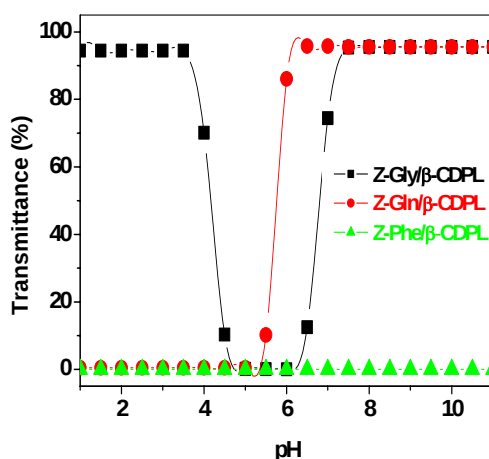
Figure 2. Transmittance changes in 1:1 mixtures of CDPL and amino acid derivatives via exposed carboxyl group of the guests.
