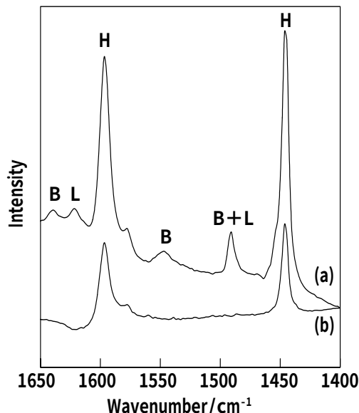
Fig. 2 FT-IR spectra of pyridine adsorbed on (a) Al-CDS-1 and (b) CDS-1 zeolites.
