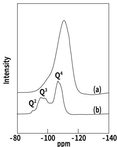
Fig. 1 ^{29}\text{Si} MAS NMR spectra of (a) Al-CDS-1 zeolites and (b) Al-PLS-1.
