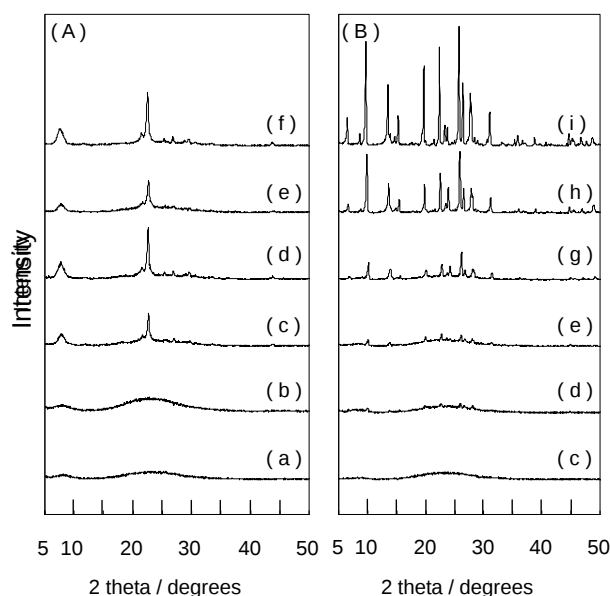
Fig. 1 XRD patterns of BEA and MOR zeolites synthesized. (A) without and (B) with NaF. Crystallization time (a) 12 h, (b) 18 h, (c) 24 h, (d) 36 h, (e) 42 h, (f) 48 h, (g) 54 h, (h) 66 h, (i) 72 h. Synthesis condition : Si/Al = 20, NaOH/AlCl 3 = 3, NaF/SiO 2 = 0 or 0.8, temp. = 443K.
