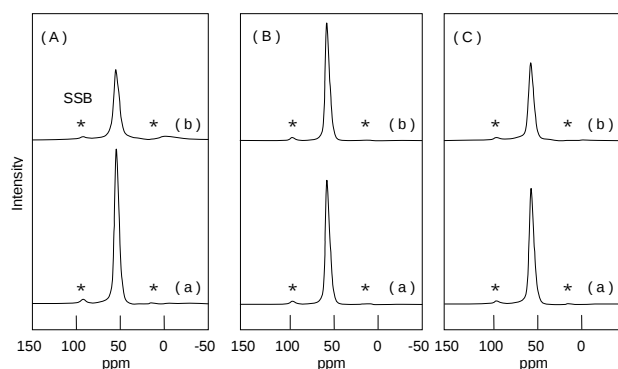
Fig. 2 27 Al MAS NMR spectra of various MOR zeolites after thermal treatment. (A) MOR ( Si/Al = 15.3 ) synthesized using the starting gel without NaF, (B) Addition time of NaF 0h, (C) Addition time of NaF 36h. (a) As-synthesized MOR was treated hydrothermally at 443K for 2 days (3 times), followed by calcination at 773K for 10 h. (b) Sample (a) was calcined at 1173K for 1 h.
