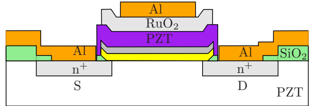
Fig.4 Schematic cross section along the A-B line in Fig.3
