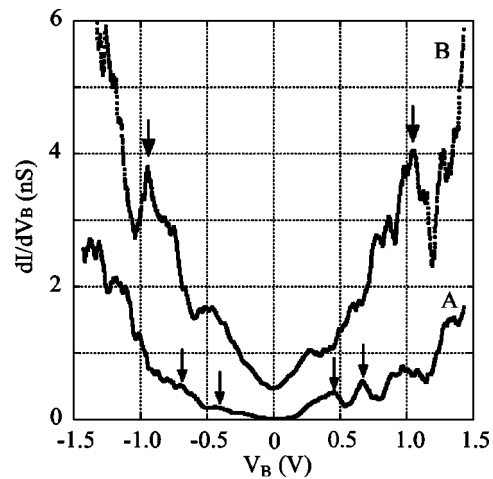
FIG. 3. Tunneling conductance dI/dV_B spectra at positions A and B in Fig. 2(b). Big and small arrows show the van Hove singularity corresponding to the metallic and the semiconducting SWNTs, respectively.
