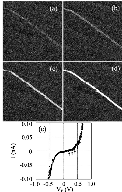
FIG. 4. Topographic current images of sample No. 2 with V_B =(a) 0.2, (b) 0.3, (c) 0.4, and (d) 0.5 V, (e) current–voltage curve.
