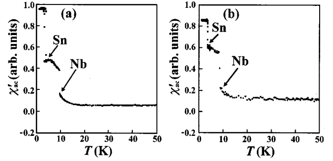
FIG. 11. ac susceptibilities of the (a) \text{Cs}_{3.2(3)}\text{C}_{60} and (b) \text{Cs}_{3.5(1)}\text{C}_{60} samples.
