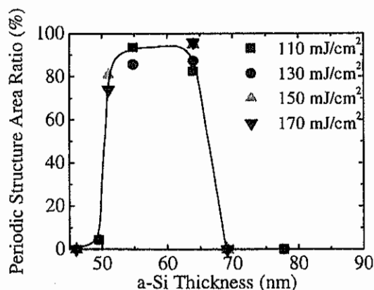
Figure 3. Dependence of the periodic structure area ratio of the non-Secco etched Si film crystallized at 2 pulses on the a-Si film thickness, where the laser energy density is 110 to 170 \text{mJ}/\text{cm}^2 .
