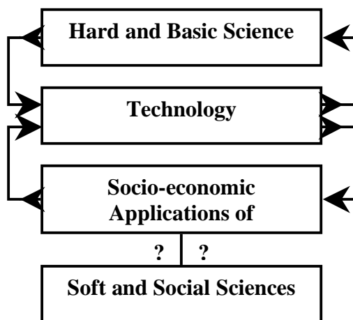
Fig. 1. Two positive feedback loops
