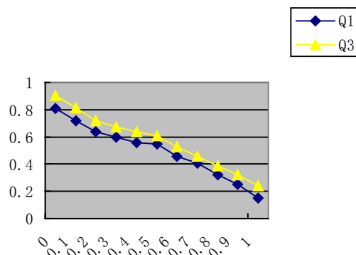
Fig.4 11 points of the precision and recall rate
