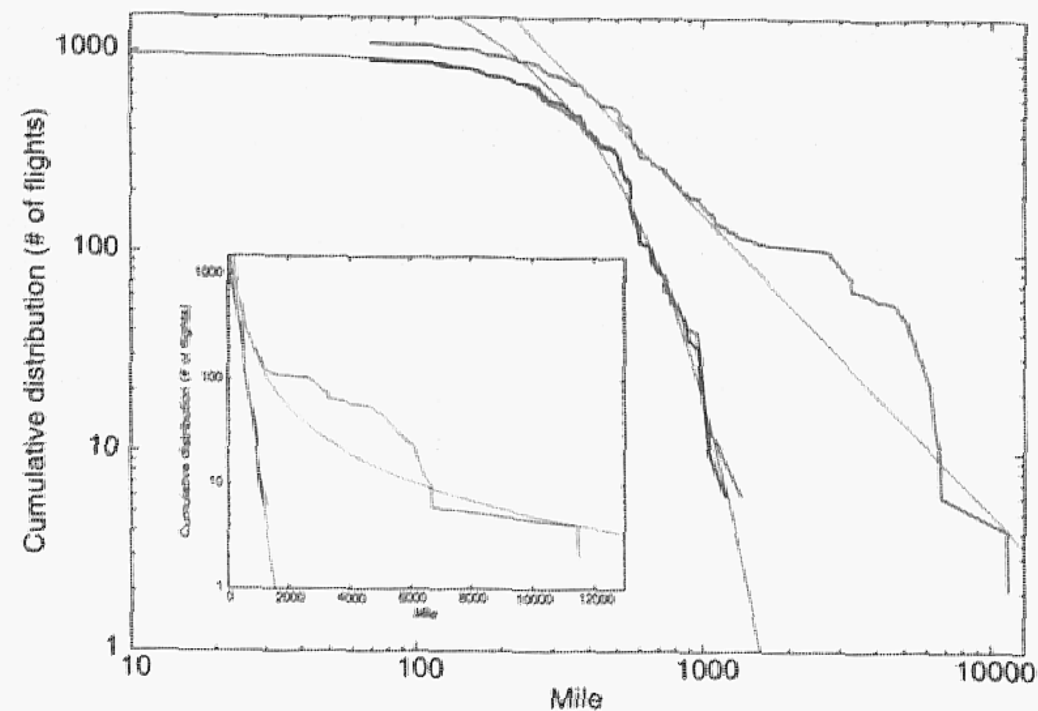
Fig. 1 Cumulative number of flights by Japanese airlines. The red, blue, and green lines correspond to domestic flights by JAL and ANA, and other flights including international flights (inset: semi-log scale). The magenta and cyan lines show the estimated exponential and power-law functions, respectively.
