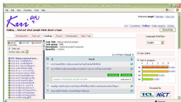
Figure 3. KUI-Polling page
