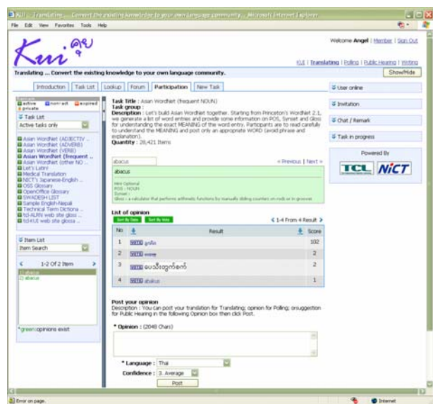
Figure 2. KUI-Translating page
