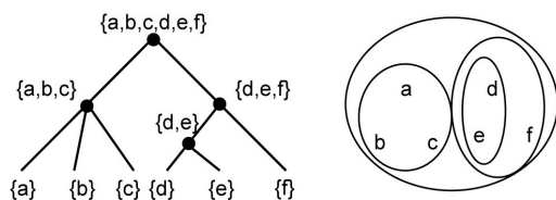
Figure 3. Tree Structure
