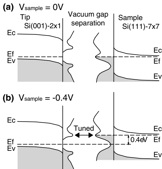
FIG. 4. Simplified tuning energy diagram of a tip of p -Si(001)-(2 \times 1) with an surface energy gap and a sample of n -Si(111)-(7 \times 7) with metallic surface states. (a) V_{\text{sample}} = 0 V, and (b) -0.4 V. We assume that the tip states are similar to those on a Si(001)-(2 \times 1) surface with asymmetric dimers. The band gap of Si is about 1.1 eV. The surface Fermi level of the Si(001)-(2 \times 1) and Si(111)-(7 \times 7) is about 0.4 and 0.7 eV above the top of valence band, respectively [25]. Thus the contact potential difference is calculated to be about -0.3 V, which is in good agreement to the measured value of about -0.27 V.
