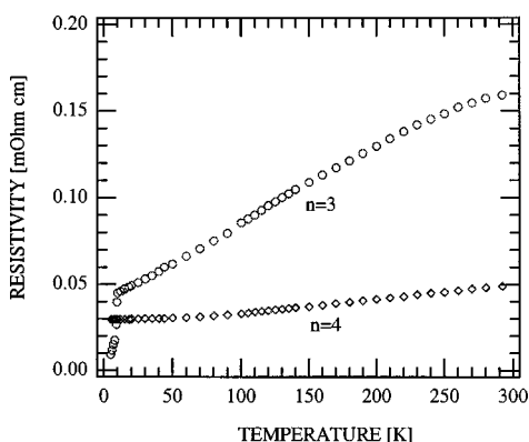
FIG. 3. Resistivity vs temperature curves for the FePc-intercalated n=3 (circles) and n=4 (diamonds) samples.
