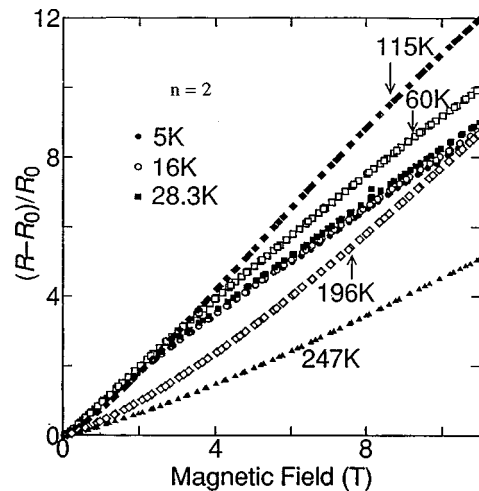
FIG. 4. MR vs applied field in the FePc-intercalated n=2 sample.
