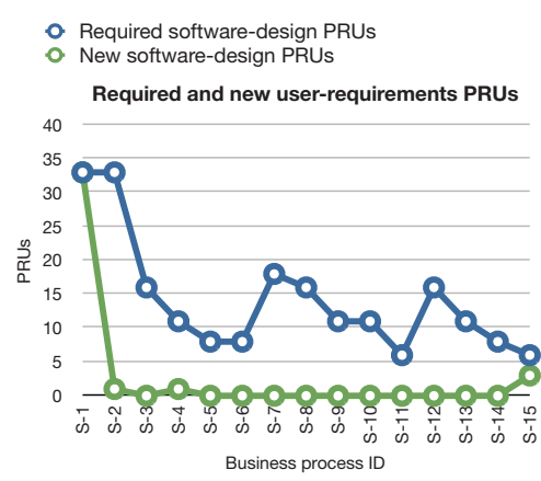
Figure 6-10. Required and new PRUs of the JBoss Seam system of Shopping-WS.
