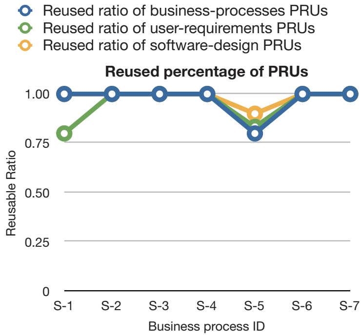
Figure 6-9. Reused ratios of the JSP system of Medical-MS.
