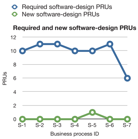
Figure 6-8. Required and new PRUs of the JSP system of Medical-SS.
