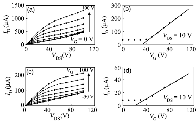
FIG. 2. (a) I_D - V_{DS} plots and (b) I_D - V_G plot for C_{60} FET device with Eu electrodes measured at 294 K just after annealing the device. (c) I_D - V_{DS} plots and (d) I_D - V_G plot for C_{60} FET devices with Eu electrodes measured at 294 K after keeping the device at 294 K for 12 h.
