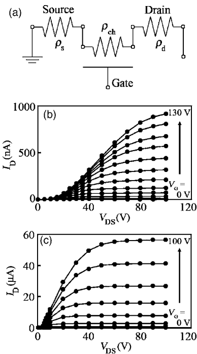
FIG. 3. (a) Circuit model for the FET device. I_D - V_{DS} plots for C_{60} FET devices with (b) Cu and (c) Pt electrodes measured at 294 K.
