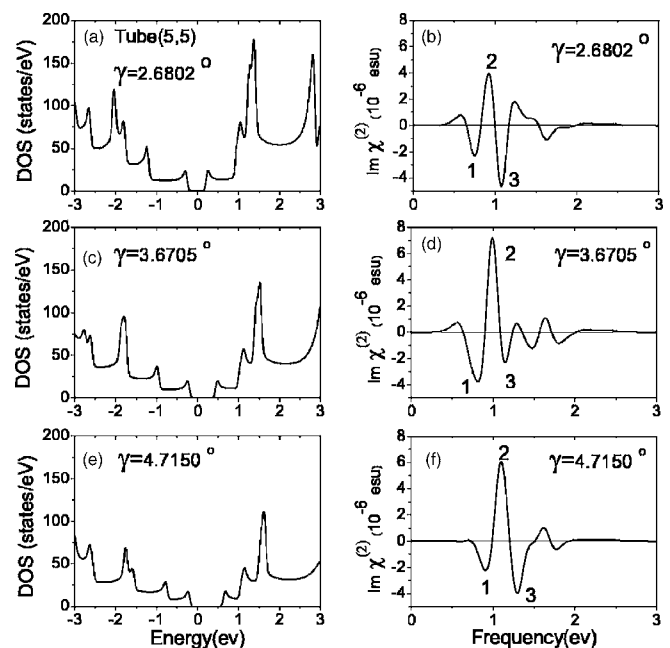
FIG. 3. Density of states (left three panels, E_f=0 ) and \text{Im } \chi_{xyz}^{(2)} (right three panels) of the (5, 5) SWNT under different torsional strains. The main peaks are listed in Table II.
