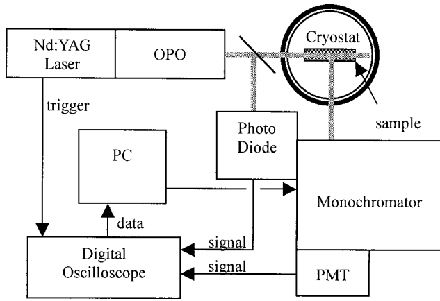
FIG. 1. Schematic diagram of FLN emission measurement system.
