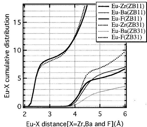
FIG. 6. \text{Eu-X} ( X=\text{Zr} , \text{Ba} , and \text{F} ) cumulative distribution of ZB11 and ZB31 fluorozirconate glasses.
