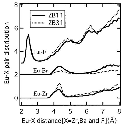
FIG. 5. Pair radial distribution function of \text{Eu-X} ( X=\text{Zr} , \text{Ba} , and \text{F} ) pairs in ZB11 and ZB31 fluorozirconate glasses.
