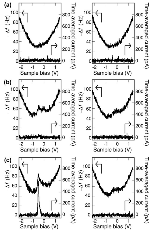
FIG. 1. \Delta f - V curves (upper) and I - V curves (lower) simultaneously taken by bias voltage NCAFS with the same tip without any change while measurements. The left column shows curves over a corner Si adatom in the faulted half of 7 × 7, and right column shows curves over an area with no Si surface atoms. (a) At a tip-sample separation of 0.9 nm. (b) At 0.5 nm. (c) At 0.4 nm. The separation values were roughly estimated, but the differences precisely evaluated. A prominent current peak is found together with a maximum \Delta f peak over the Si atom in (c).
