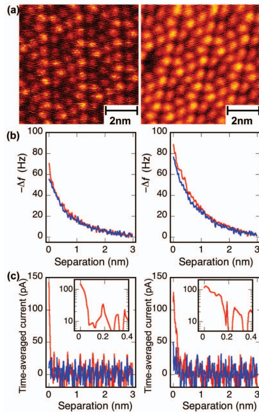
FIG. 2. (Color) \Delta f and time-averaged current I versus tip-sample separation at V=-0.5 and -0.2 V, in left column and right column, respectively. Red curves over a corner Si adatom and blue curves over an area with no Si surface atoms. (a) Current I images simultaneously obtained at \Delta f=58 and 82 Hz for -0.5 and -0.2 V, respectively. (b) \Delta f -distance curves. (c) I -distance curves simultaneously obtained with (b). Insets show log-scaled I around close separation.
