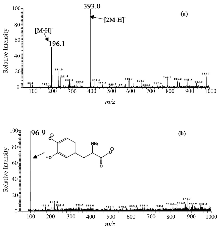
Fig. 5. (a) Negative ion ESI mass spectrum of DOPA. (b) Negative ion ESI mass spectrum of DOPA and CuCl_2 .
