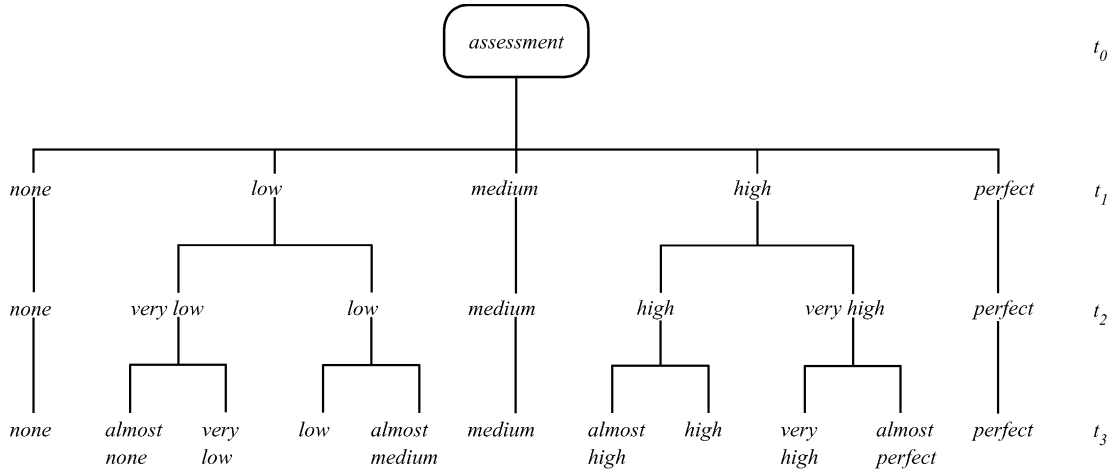
Fig. 2. Linguistic hierarchy T_{assessment} .
