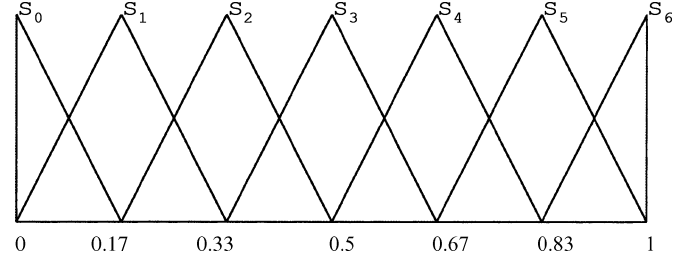
Fig. 1. Linguistic term set.
