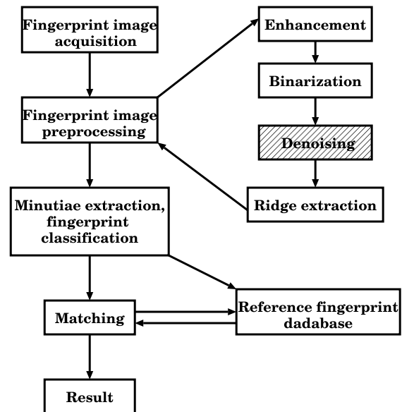
Fig. 1 A flowchart showing different phases of fingerprint analysis. The highlighted module shows the area of our work.
