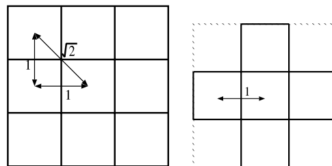
(a) 3 \times 3 SE: d = \sqrt{2} (b) Cross SE: d = 1
