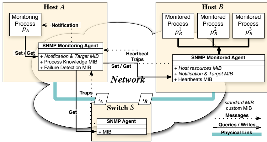
Figure 2: SNMP Usage
